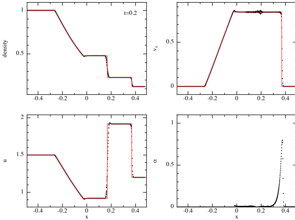
Figure 9. As in Figure 8, but with code defaults for all dissipation terms ( \alpha^{AV} \in [0, 1] ; \alpha_u = 1 ). These leave more noise in the velocity field behind the shock but provide second order convergence in smooth flow. The lower right panel in this case shows the resultant values for the viscosity parameter \alpha^{AV} .
