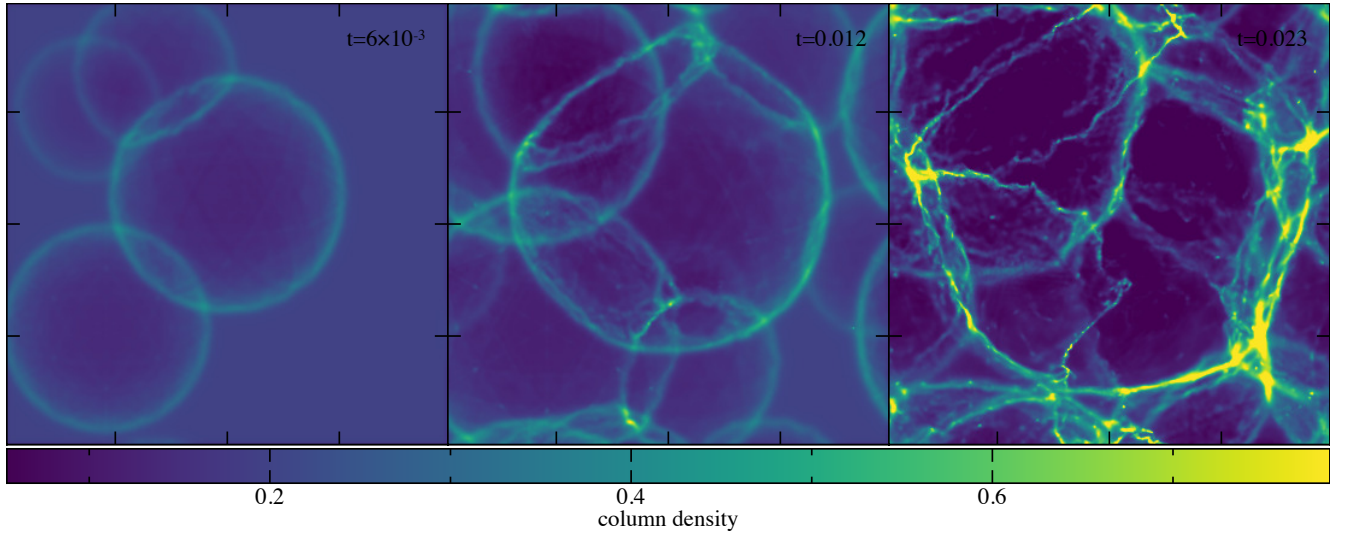
Figure 37. Balsara-Kim supernova-driven turbulence, showing column density at three different times at a resolution of 64 \times 74 \times 78 particles. Supernovae are injected every 0.00125 in code units, leading to a series of interacting blast waves. Interstellar chemistry and cooling is turned on, producing a dense filaments in a turbulent interstellar medium.
