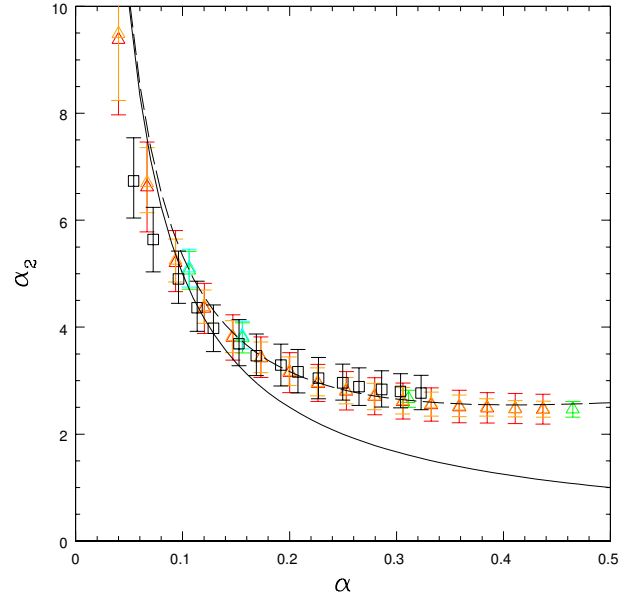
Figure 21. Warp diffusion rate as a function of disc viscosity, showing the PHANTOM results as compared to the non-linear theory of Ogilvie (1999) (dashed line). The linear prediction, \alpha_2 = 1/(2\alpha) , is shown by the solid line, highlighting the agreement of PHANTOM with the non-linear theory. Colouring of points is as in Figure 20. Figure taken from Lodato & Price (2010).
