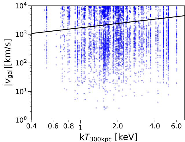
Fig. 3. Magnitude of the rest-frame velocity of cluster galaxies, Eq. (1), as a function of cluster temperature. Each dot is one galaxy, and some galaxies appear in the fields of multiple clusters. The black line shows the cut, Eq. (2), that separates the lower signal population from a projected background. Points above the black line are disregarded in our analysis.
