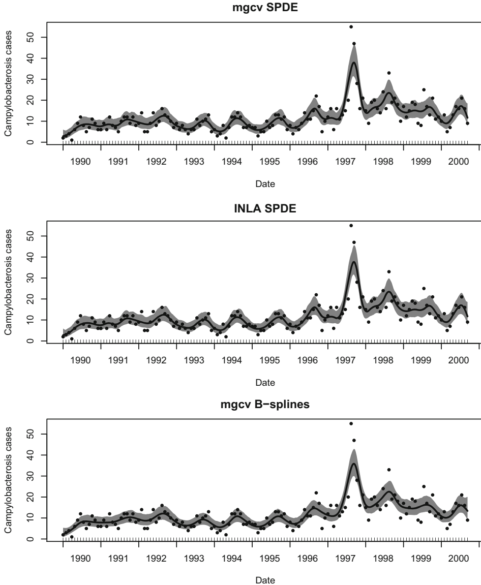
Figure 3. Campylobacteriosis cases modelled using: a Matérn basis-penalty smoother fitted with \text{mgcv} (top), a Matérn SPDE fitted with \text{R-INLA} (middle), a B-spline basis-penalty smoother fitted using \text{mgcv} (bottom).
