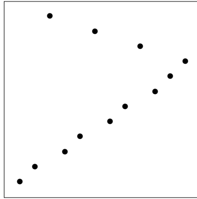
\phi = (1, 2, 12, 3, 4, 11, 5, 6, 10, 7, 8, 9)
