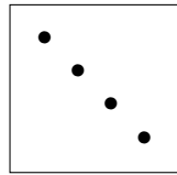
\alpha = 4321
