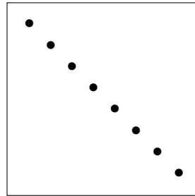
\theta = 87654321
