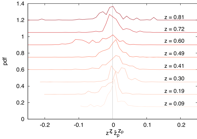
Figure 5. The PDFs found by the BDT method for randomly selected galaxies across the redshift range, centred on the photometric redshift.
