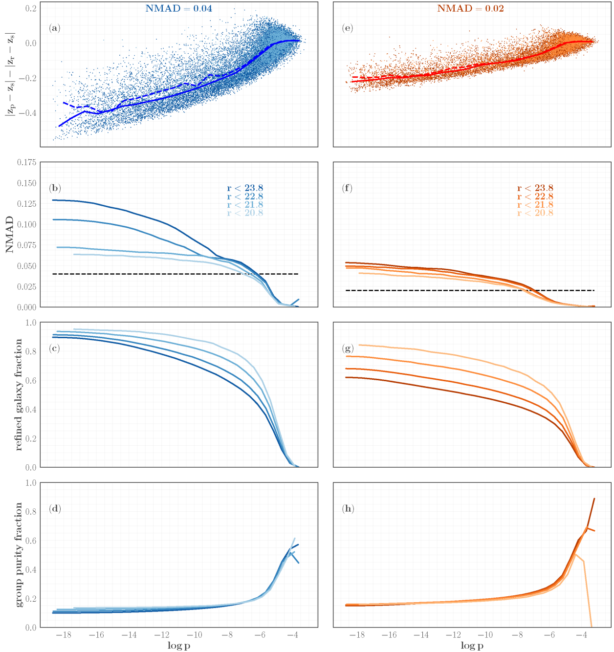
Figure 6. Post-refinement assessment of the DESI data, with intrinsic NMAD = 0.04 (left-hand panels) and 0.02 (right-hand panels) as a function of assignment probabilities.
