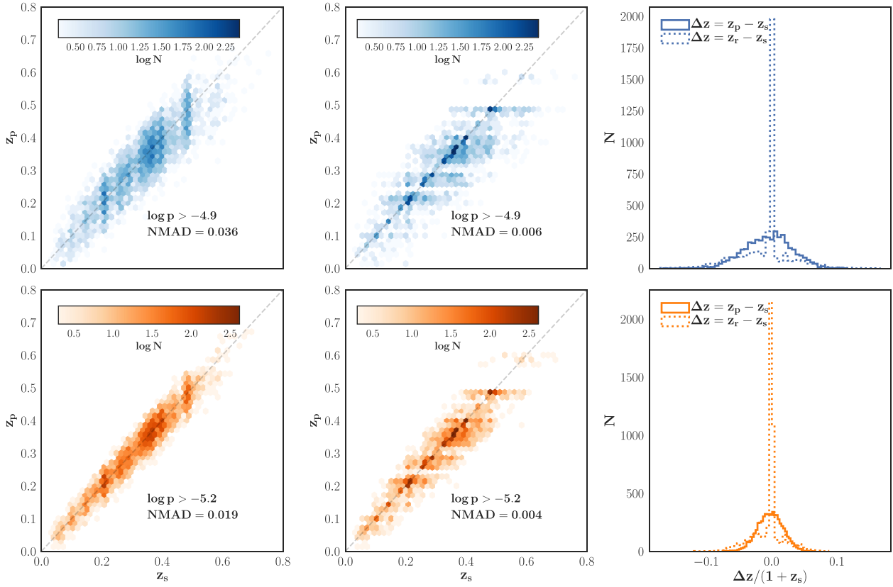
Figure 8. Photometric (left-hand panels) and refined (central panels) redshifts correlations with spectroscopic redshifts, and distributions of scaled-biases before and after refinement (right-hand panels) for the DESI data with intrinsic NMAD = 0.04 (top row) and 0.02 (bottom row).
