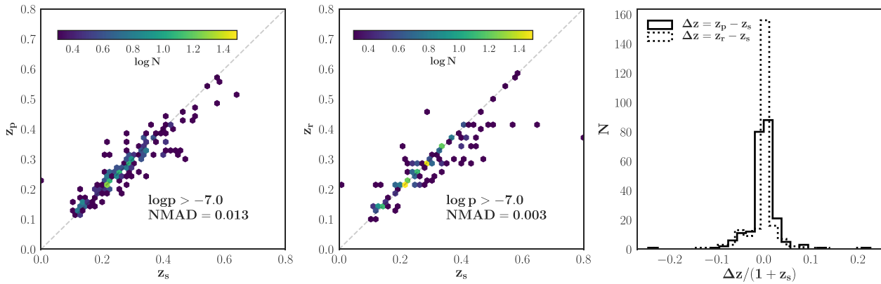
Figure 11. G15QRDEG-DEEP spectroscopic versus photometric (left-hand panel) and refined (centre panel) redshifts, and distributions of scaled-biases before and after refinement (right-hand panel).
