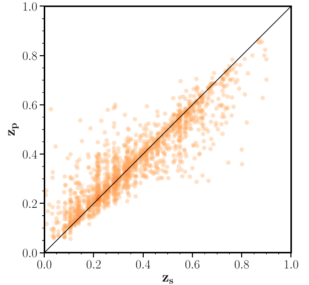
Figure 4. Spectroscopic versus photometric redshifts of the G15SQRDEG-DEEP galaxies produced by the BDT method.
