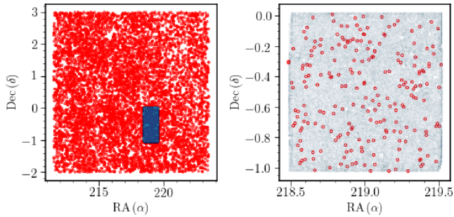
Figure 1. Galaxy and group samples. Left: position of KiDS galaxies in G15SRDEG region (blue region) and overlapping galaxy groups (represented by the positions of the central galaxies) from the GAMA group catalogue (red dots) in the entire G15 region shown in the equatorial coordinates. Right: zoomed-in version of the left-hand panel at G15SRDEG region. RA and Dec. are equatorial angles in degrees.
