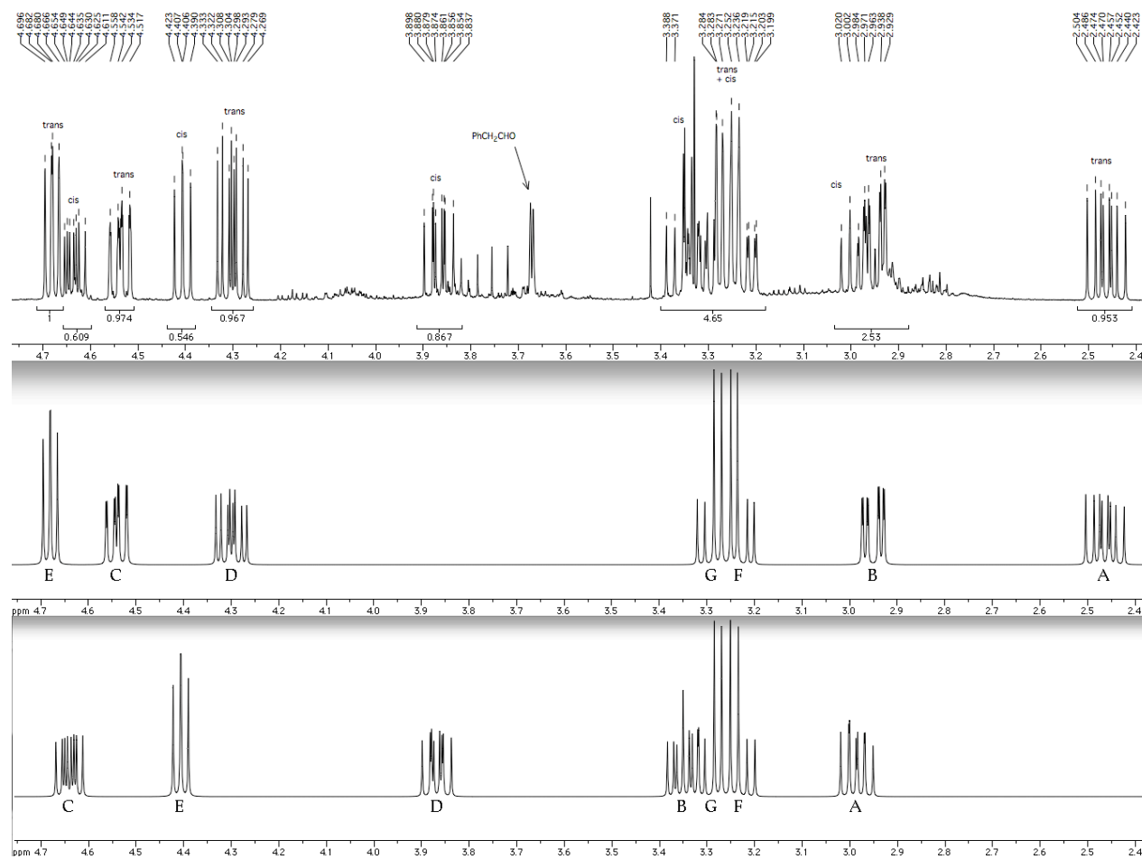
Figure 1. Aliphatic region of the ^1\text{H} NMR spectrum of 7 showing (top) experimental spectrum for mixture of cis and trans -isomers, (middle) simulation for trans - 7 , and (bottom) simulation for cis - 7 , both using values given in Table 1.
