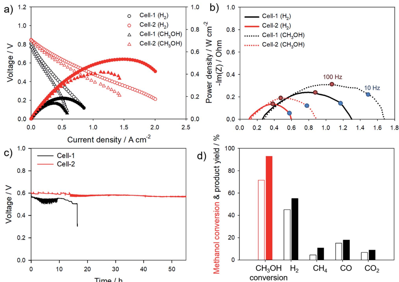
Fig. 6 (a) I-V curves of the Cell-1 and Cell-2, (b) impedance spectra of the Cell-1 and the Cell-2 at 550 °C with H 2 and CH 3 OH fuel. (d) Gas chromatography (GC) analysis of product composition of the Cell-1 and Cell-2 anode with 10 000 \text{cm}^3\ \text{h}^{-1}\ \text{g}_{\text{cat}}^{-1} GHSV CH 3 OH at 550 °C.
