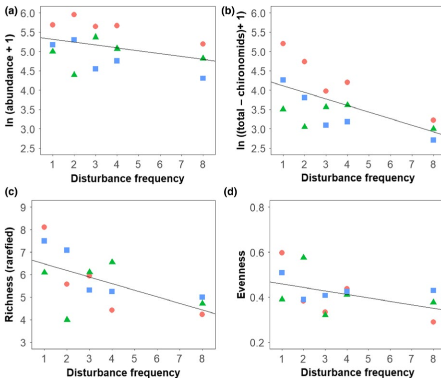
FIGURE 2 The influence of the frequency of streambed-moving disturbance on diversity. (a) Total abundance of invertebrates, slope = -0.07 , p = 0.048 ; (b) abundance of all invertebrates barring the dominant taxon (chironomids) within in-situ stream channels, slope = -0.18 , p = 0.002 ; (c) rarefied richness, slope = -0.29 , p = 0.017 ; (d) Pielou's equitability, slope = -0.02 , p = 0.098 . Symbols and colors indicate experimental block: upstream (red circle), mid-stream (green triangle) and downstream (blue square)
