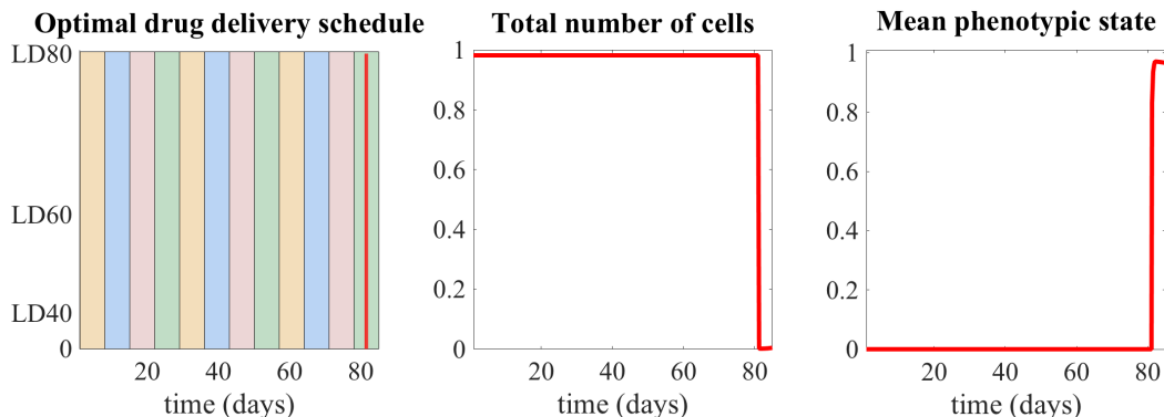
Figure 12: Optimal dosing regimen for 12 therapy cycles of 1 week with 3 days of rest per week with the goal being to minimise the total number of cells at the end of the treatment. Dynamics of the total number of cells \rho(t) in units of 10^8 (central panel) and the mean phenotypic state of the cell population \mu(t) (right panel) under the optimal drug delivery schedule u(t) (left panel) which is obtained by solving numerically the optimal control problem given by equation (5.6), with J defined by equation (5.2), subject to the dynamic constraints given by the system of differential equations (3.9) and the control constraints given by equation (5.8). Simulations have been carried out over a time window corresponding to 84 days using the parameter values listed in Table 1, the values of the terms \rho^0 , f^0 and \mu^0 given in equation (4.1) and the additional assumptions given by equation (5.10). The simulations refer to a treatment protocol which consists of 12 therapy cycles of 1 week whereby 4 days of therapy must be followed by 3 days of rest, and there is a maximum amount of drug that can be administered over the 4 days of therapy, which is the same for all the therapy cycles. Therefore, we have specified the constraint given by equation (5.8) as in equation (5.12) with the value of C corresponding to the LD80. The coloured rectangles in the left panel highlight the different therapy cycles.
