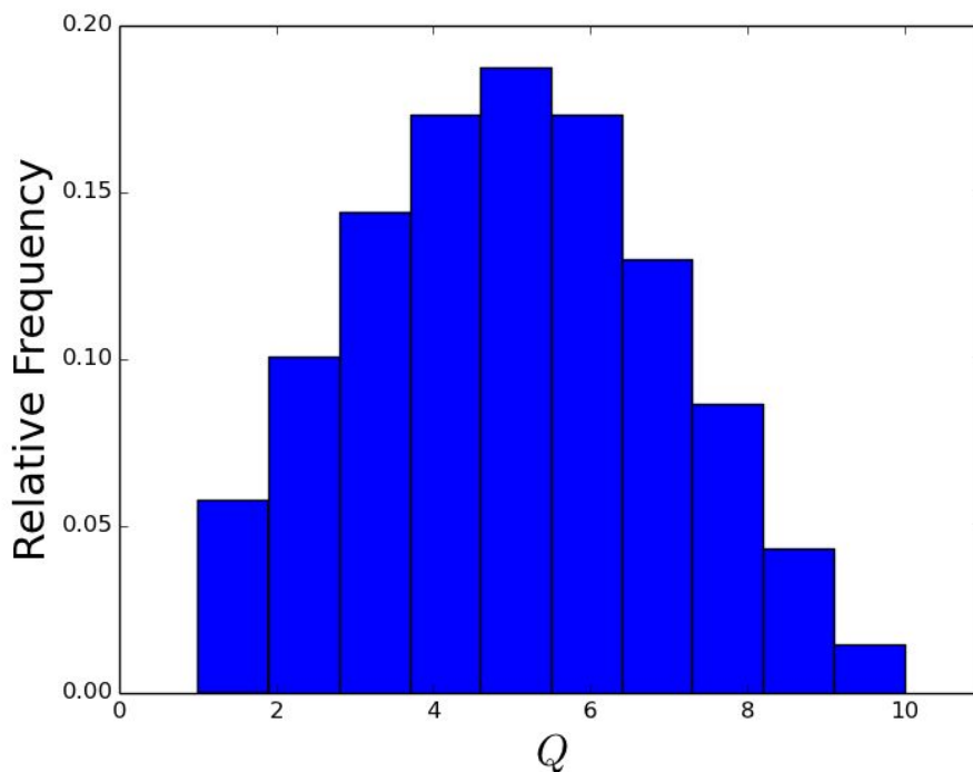
Figure 2: The distribution of all possible Q scores in the Rio 2.0 scheme
