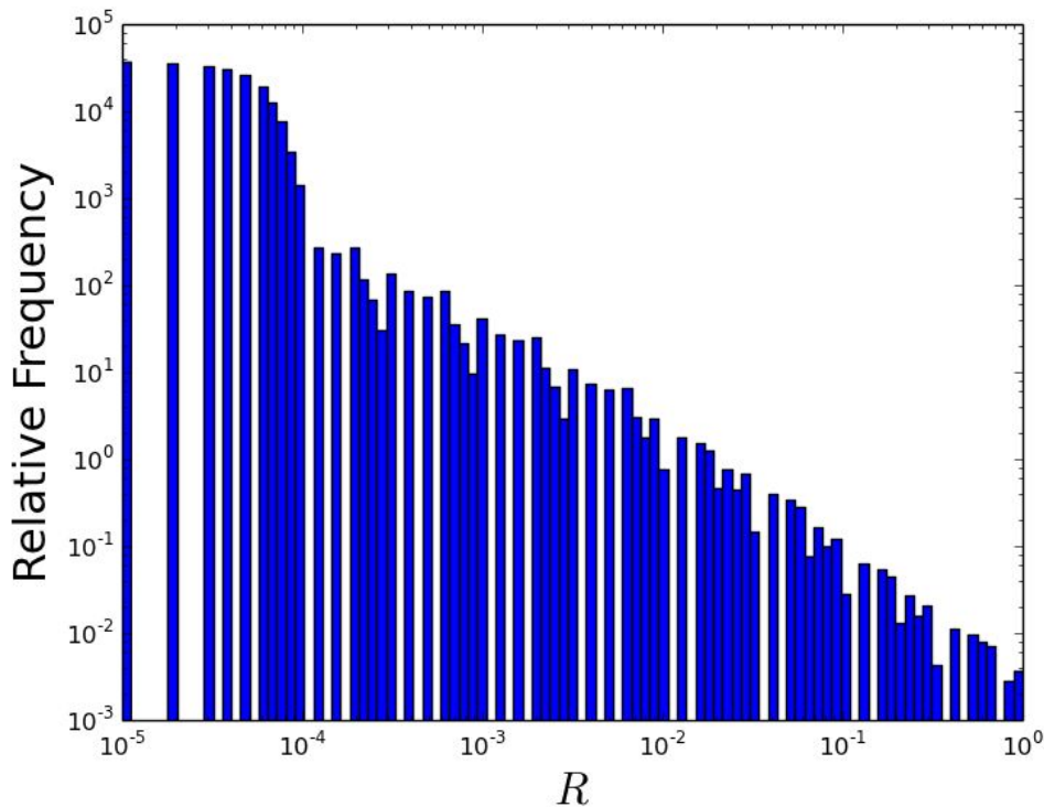
Figure 5: The distribution of Rio scores in the Rio 2.0 scheme
