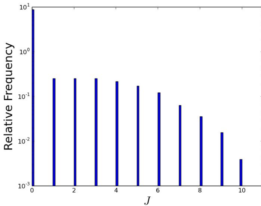
Figure 3: The distribution of J scores in the Rio 2.0 scheme.
