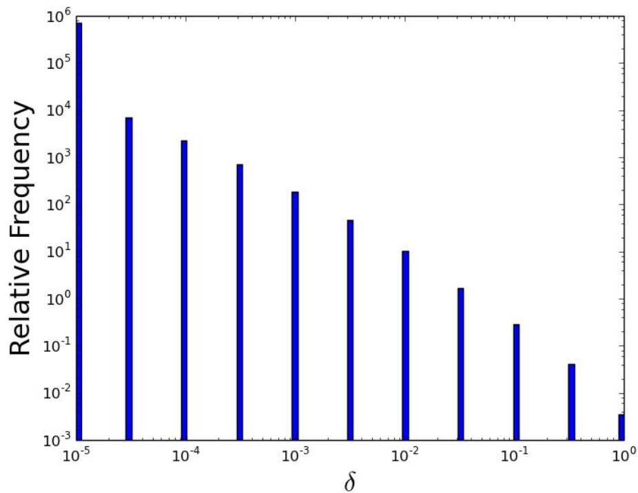
Figure 4: The distribution of delta scores in the Rio 2.0 scheme.
