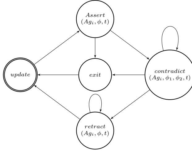
Fig. 1: Protocol Rules
