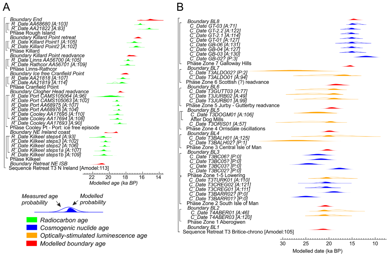
Figure 12. Bayesian models for the dating of ice retreat across (A) north-east Ireland and (B) the north-east Irish Sea Basin. The model structure shown uses OxCal brackets (left) and keywords that define the relative order of events (Bronk Ramsey, 2009a). Each original distribution (hollow) represents the relative probability of each age estimate with posterior density estimate (solid) generated by the modelling. Shown are ^{14}\text{C} ages (green), OSL ages (orange), CN ages (blue) and modelled boundary ages (Red). Outliers are denoted by '?' and their probably (P) of being an outlier indicated by low values <5 (95% confidence). Model agreement indices for individual ages show their fit to the model with >60% the widely used threshold for 'good' fit (Bronk Ramsey, 2009a). [Colour figure can be viewed at wileyonlinelibrary.com ]
