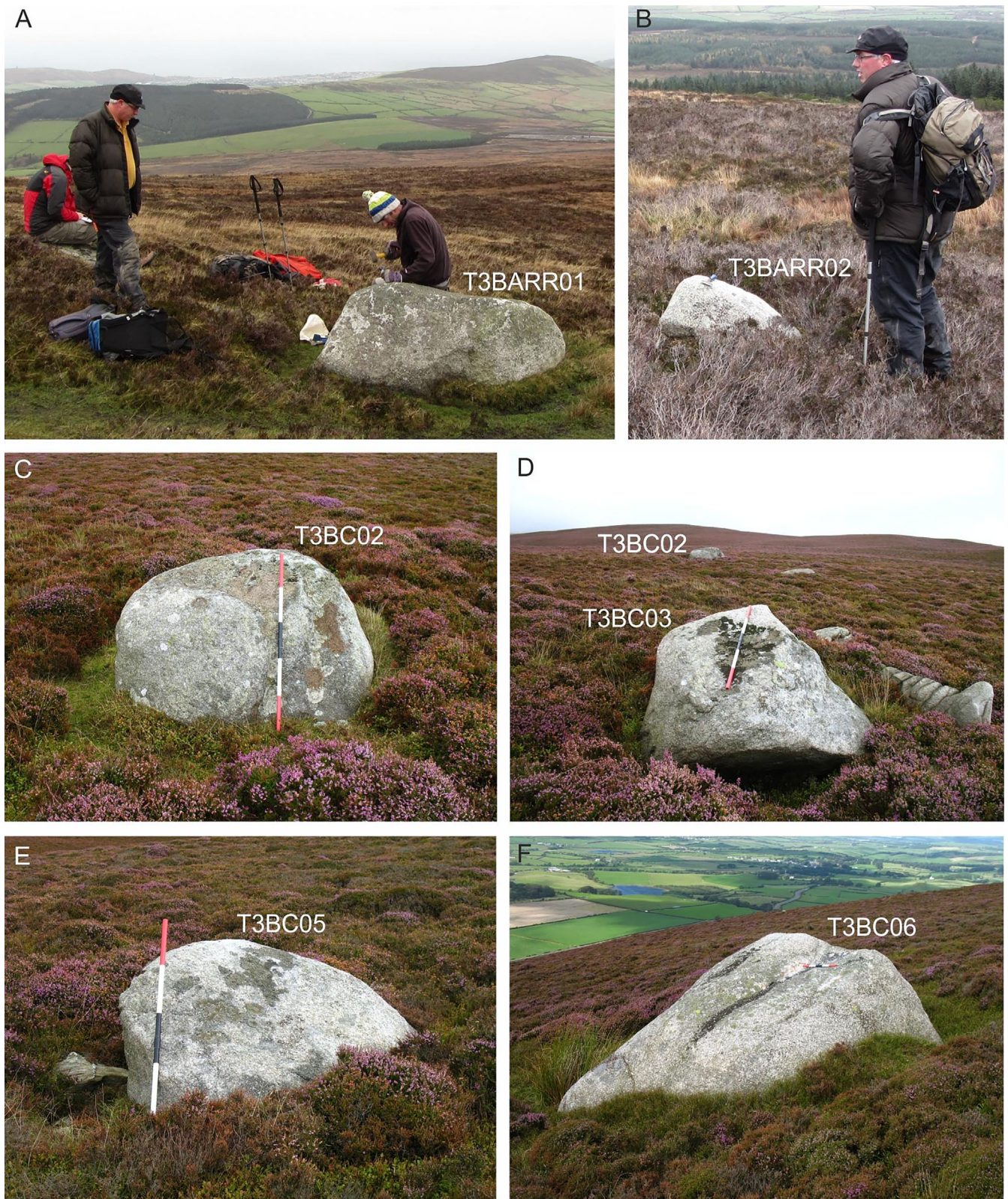
Figure 4. Cosmogenic nuclide samples: A, T3BARR01 from the summit of South Barrule; B, T3BARR02 from the flanks of South Barrule on the Isle of Man; C–F, samples T3BC02, T3BC03, T3BC05 and T3BC06 from Black Combe in western Cumbria, NW England. [Colour figure can be viewed at wileyonlinelibrary.com ]
