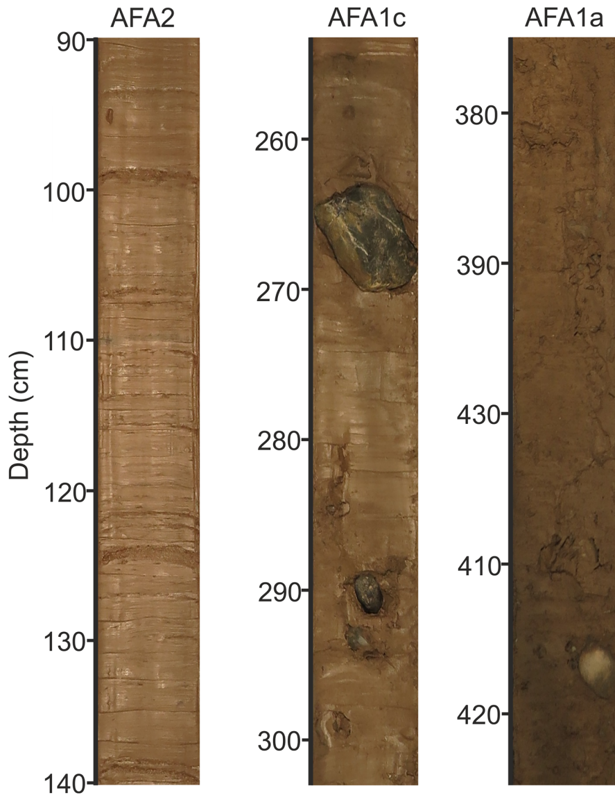
Figure 11. Lithofacies examples from key acoustic facies sampled from vibrocore JC106-084VC from line y^2 - y^3 (Fig. 10D). [Colour figure can be viewed at wileyonlinelibrary.com ]
