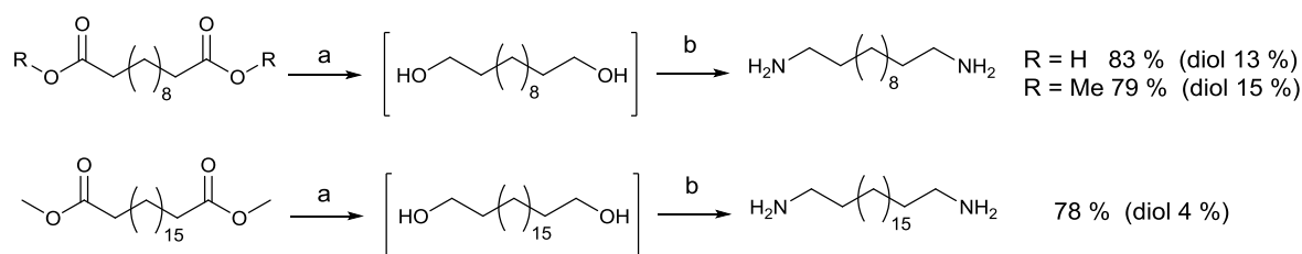
Scheme 1. a [Ru(acac) 3 ] (2 mol%), triphos (4 mol%), MSA (2 mol%), 1,4-dioxane (7.5 mL), substrate (1.25 mmol), distilled water (5 mL), H 2 (10 bar), 220 °C, 20 h. b 1,4-dioxane (12.5 mL), aq. ammonia (35 %, 30 mL), H 2 (10 bar), 220 °C, 20 h.
