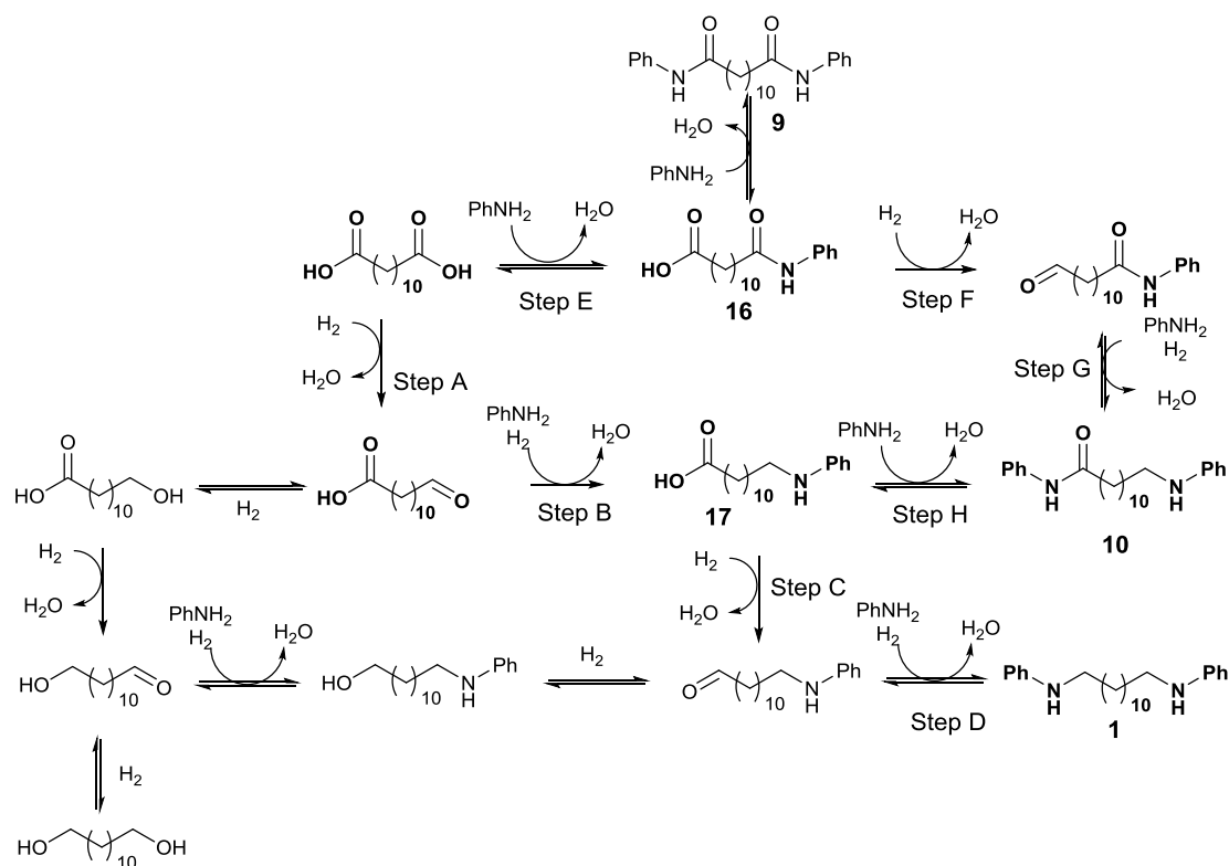
Scheme 2. Proposed reaction pathway for the hydrogenation of 1,12-dodecanedioic acid in the presence of aniline to give 1 (Steps A-D and/or E-H, C, D, intermediates are bold), numbered compounds have been identified as being formed during the reaction; the reductive amination of 1,12-dodecanediol with aniline to give 1 (bottom) and the hydrogenation of 1,12-dodecanedioic acid to 1,12-dodecanediol (left hand side). The sequential reaction using ammonia proceeds through the hydrogenation to dodecanediol followed by reductive amination.
