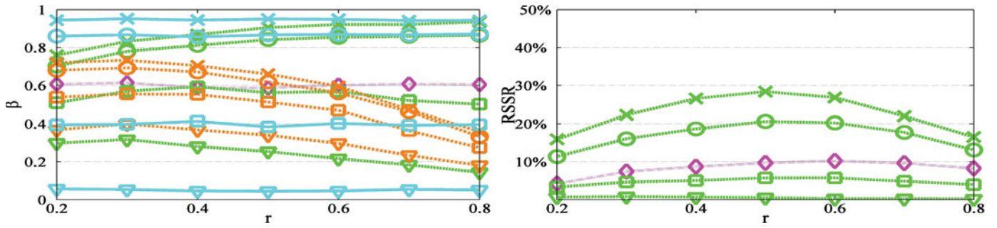
Figure 1. Power (left panel) and RSSR (right panel) versus sample allocation ratio. We plot the sequential \chi^2 -test (magenta \bullet\circ\cdot ) and the z^* (green -- line), sequential z (cyan - ), and z^+ (orange - \cdot - ) tests with first stage/fixed/first step weighting vector 0 ( \times ), 30^\circ ( \circ ), 60^\circ ( \square ) and 90^\circ ( \nabla ) angle to the optimal. The remaining design parameters are J = 2 , K = 10 , \alpha = 0.05 , \alpha_{1,1} = 0.01 , \alpha_{0,1} = 1 , n_T = 60 , n_0 = 0.5n_1 , D_{\mu, \Sigma} = 0.65 .
