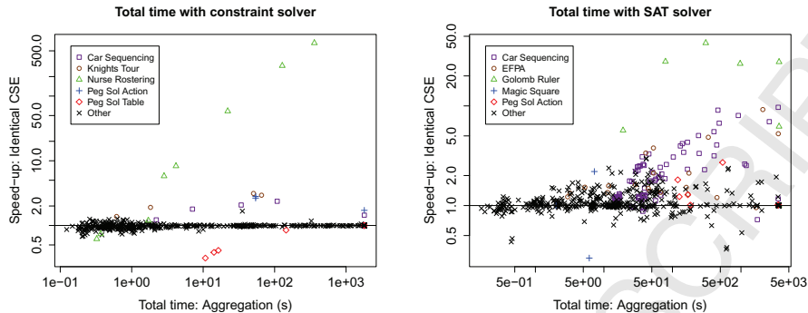
Figure 6: Comparing Identical CSE to Aggreg (total time) with the CP solver (left) and the SAT solver (right). Axes are the same as Figure 3.
