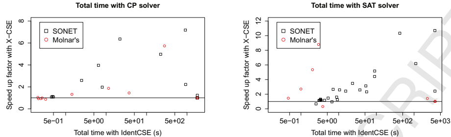
Figure 10: Comparing X-CSE to IdentCSE for SONET and Molnar's Problem total time, with the CP solver (left) and the SAT solver (right).
