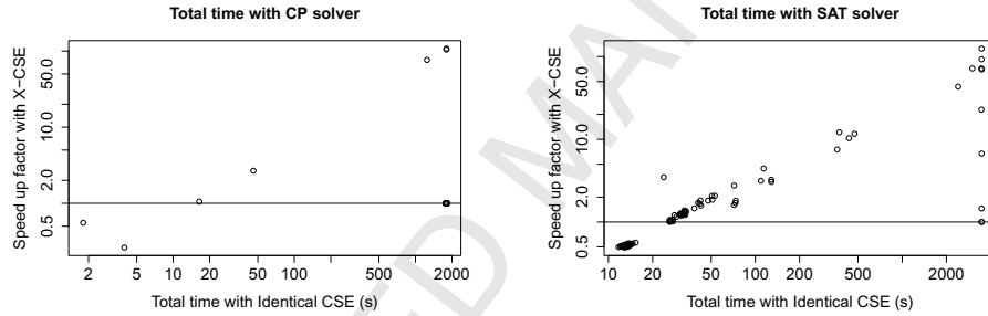
Figure 13: Comparing X-CSE to IdentCSE for Car Sequencing total time, with the CP solver (left) and the SAT solver (right).
