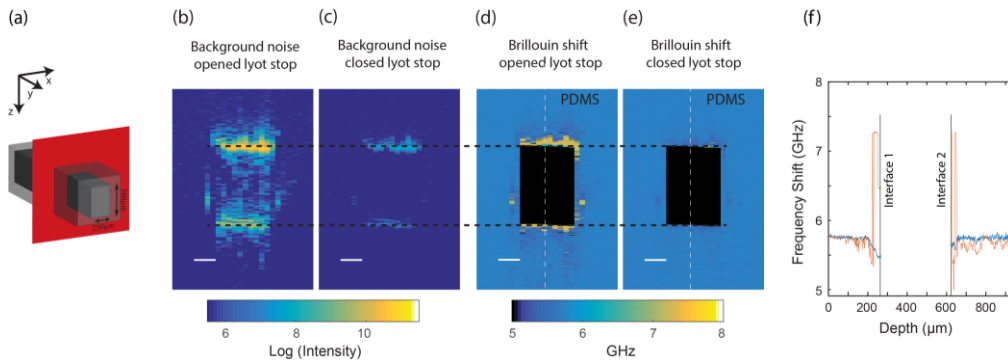
Fig. 4. Brillouin imaging of a micro-fluidic channel: (a) Illustration of the PDMS micro fluidic channel (width=250 μm, height=360 μm). Scanning was performed across the XZ plane highlighted in red. Background noise levels defined as the average intensity value between the Brillouin peaks with (b) the Lyot stop widely open and (c) with a closed Lyot stop (scale bar = 100 μm). The noise from the interfaces was nearly removed for the latter. False color bar indicates camera counts on log scale. Brillouin shifts recorded with (d) an open Lyot stop and (e) a closed Lyot stop. For the former there are clear artifacts up to 50 microns away from the interfaces, whereas the latter show a continuous Brillouin shift up to the interface between air and PDMS. (f) Line plots of the Brillouin shift measurements across the central part of microfluidic channel denoted by a dashed line in Figs. 4(d) and 4(e), for an opened Lyot stop (red) and a closed Lyot stop (blue).
