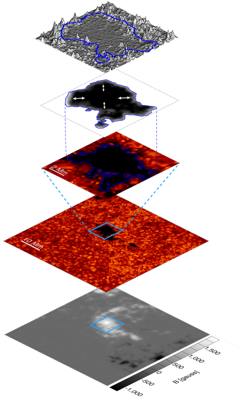
Figure 5. This stack image shows the basis of our designation of a sausage surface mode in this pore. The bottom panel shows the LOS magnetogram from HMI indicating the magnetic field of the pore and the sharp boundary in terms of magnetic field at the pore's edge. Above this is the full FoV ROSA G-band image showing the photospheric appearance of the pore taken on 2011 December 10. The blue box indicates the expanded region shown in the three top panels. The expanded G-band image has blue contours indicating the pore boundary established for that particular frame. Above this is the time-averaged pore boundary map showing the variation in boundary location during our observation sequence, where the arrows indicate the sausage mode oscillations present. The top panel is a two-dimensional power plot of the power across the pore obtained with wavelet transforms of the data filtered at a frequency of \sim 4.6 mHz. The blue contour shows the time average pore boundary location. Peaks in power at this boundary indicate a sausage mode is observed at this frequency.
