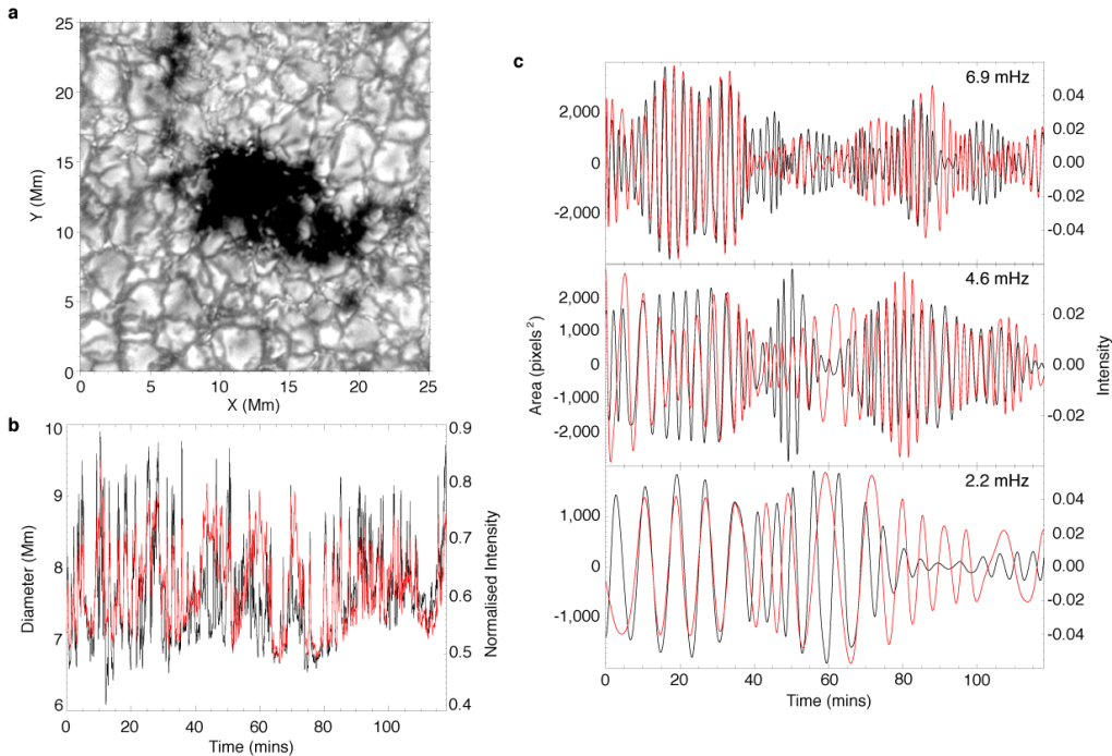
Figure 8. The images presented here help to verify the decision that the G-band continuum filter is an acceptable continuum bandpass for studying sausage oscillations in photospheric pores. Panel a shows a sub-field of data taken with the 4170 Å continuum filter for the 2011 December 10 dataset used in the paper. This is the same sub-field as depicted in Figure 4. Panel a shows the visual similarities between the two filters. Panel b and c mirror plots seen in Figure 2. Panel b shows the area ( black ) and intensity ( red ) signals for the pore over the duration of the observing sequence for the 4170 Å filter. The difference in intensity signals between the G-band and 4170 Å continuum filters is less than 2%. Oscillations with the same period as those previously observed with the G-band filter were observed in the 4170 Å filter area and intensity signals as well. Panel c shows the associated IMFs for these three oscillations in the 4170 Å continuum images. Again, black represents the area and the red curves show the IMFs associated with the intensity signal. A similar phase relationship is observed for these signals as those observed with the G-band continuum images.
