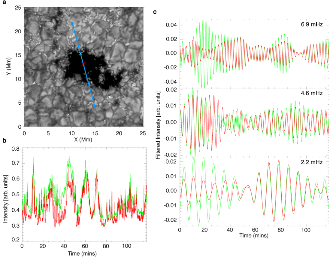
Figure 4. Panel a shows a sub-field of the pore under analysis in Figure 2 with the blue line indicating the cross-cut used to make the images in Figure 3. The red and green crosses indicate the locations used to plot the subsequent light curves shown in panel b and c for a pixel at the center of the pore ( red ) and at the pore boundary ( green ). Panel b shows the unaltered intensity curves for these locations with the color of the line consistent with the crosses in the panel above. Panel c shows the results of filtering these light curves as described in the main text over the whole time sequence of the dataset. Again, the colors of the plots are consistent across all panels. It is clear from the filtered plots that there is significant amplitude in intensity oscillations at both the pore boundary and the interior across all three sampled frequencies. The power plots in Figure 3 panel b of the main text are created using frames between \sim 35 – 65 minutes, \sim 66 – 84 minutes and \sim 1 – 29 minutes, from the start of the observing sequence for the 6.9 mHz, 4.6 mHz, and 2.2 mHz oscillations, respectively.
