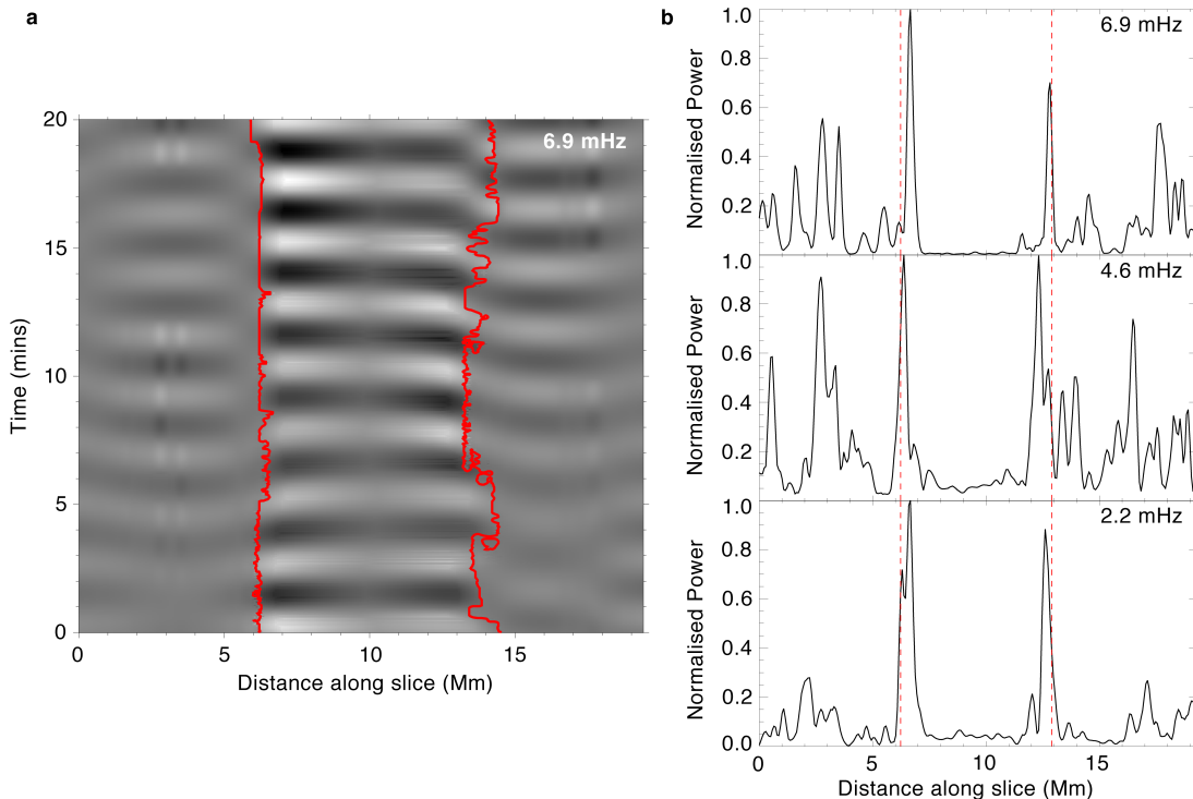
Figure 3. Coherent oscillatory behavior is identified throughout the pore for data from 2011 December 10, and is occurring with a number of distinct frequencies. Panel a shows a temporally filtered (at \sim 6.9 mHz) time-distance diagram taken from a slice across the pore. The analysis reveals a clear, spatially coherent oscillatory pattern within the pore boundaries (outlined in red ). The time axis of the plot is clipped to 20 minutes to ensure that the small pixel-to-pixel amplitude variations across the pore are evident. The time window is established by using EMD and wavelet analysis to determine when a clear in-phase wave is present in the filtered area and intensity signals (Figure 2). In the above plot, the 20-minute window equates to the time period of 35 minutes to 55 minutes from the start of data acquisition and represents the time period over which the corresponding plot in panel b is derived. The right-hand panels b display the normalized Fourier power for three distinct oscillatory frequencies of the pore. The power is seen to peak close to the temporally averaged location of the pore boundary ( red dashed lines ), supporting their characterization as a surface mode. Figure 4 indicates the cut used to make these plots and demonstrates the process of filtering lightcurves at both the pore boundary and pore center for the various oscillations present here.
