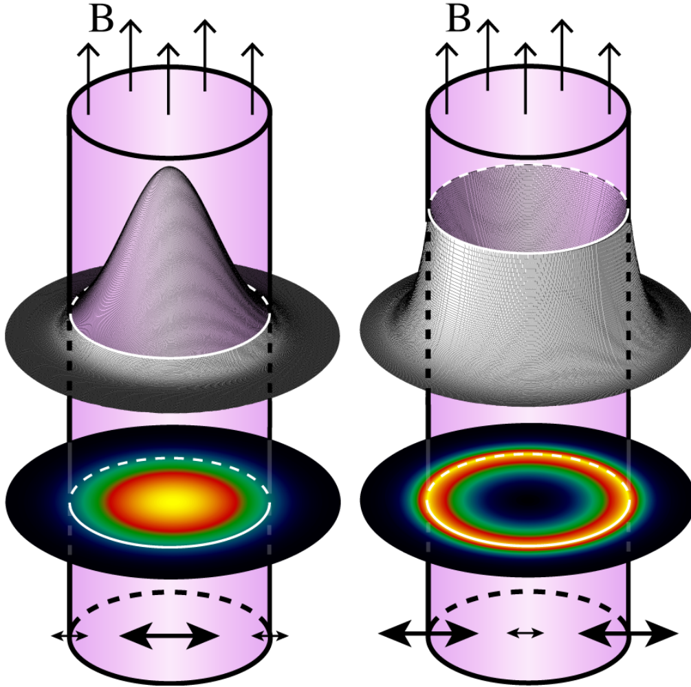
Figure 1. A simplified representation of magnetic flux tubes is shown with the arrows at the top indicating the magnetic field, \mathbf{B} . Plasma parameters (e.g., magnetic field, density) of the internal and external plasma differ. Magnetic flux tubes that support the MHD sausage mode are subject to a periodic variation in pressure and area (with these oscillations depicted by the arrows at the bottom). The surface plots (upper images) demonstrate the spatial structure of the pressure perturbation amplitude, which can have two distinct distributions. The amplitude of the body mode (left) is maximal at the central, inner part of the flux tube with the power decaying close to the boundary. On the other hand, surface modes (right) are maximal at the tube boundary defined by the sharp changes in equilibrium quantities modeled as a discontinuity. The two-dimensional projection of the power is also demonstrated by the colored disks, and can be compared to the observed distributions.
