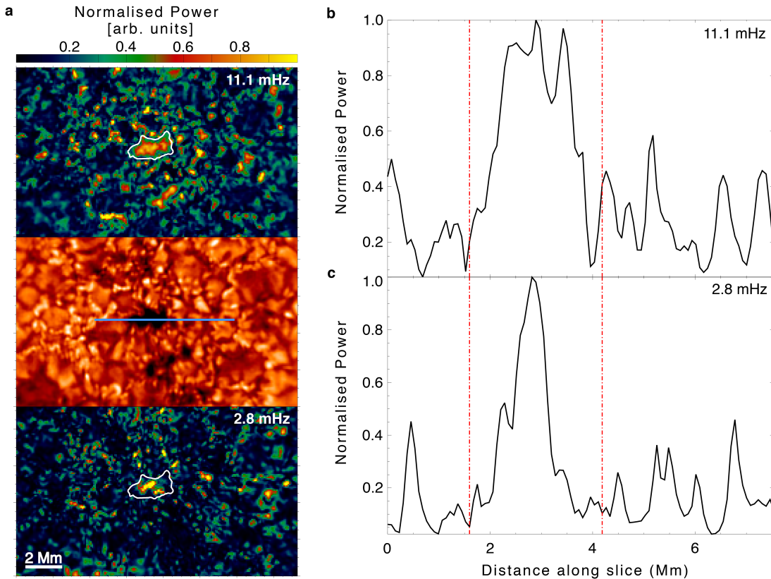
Figure 6. The oscillatory signals of a near elliptical pore (central panel in a ), observed on 2012 September 30, reveal concentrations of power peaking at the center of the pore. The upper and lower panels of a show the wavelet power for the pore filtered at a central frequency of 11.1 mHz and 2.8 mHz, respectively. White contours in these power maps show the time averaged boundary location for the pore. Images in b display the corresponding one dimensional cross cuts for the two power maps in a . Cuts were taken from the position marked by the blue line in the central panel of a . The red dashed lines in b indicate the pore boundary. Again, it is evident in these cross cuts, as with the two-dimensional power plots, that power peaks within the center of the pore and decays at the boundaries, which is synonymous with the body mode.
