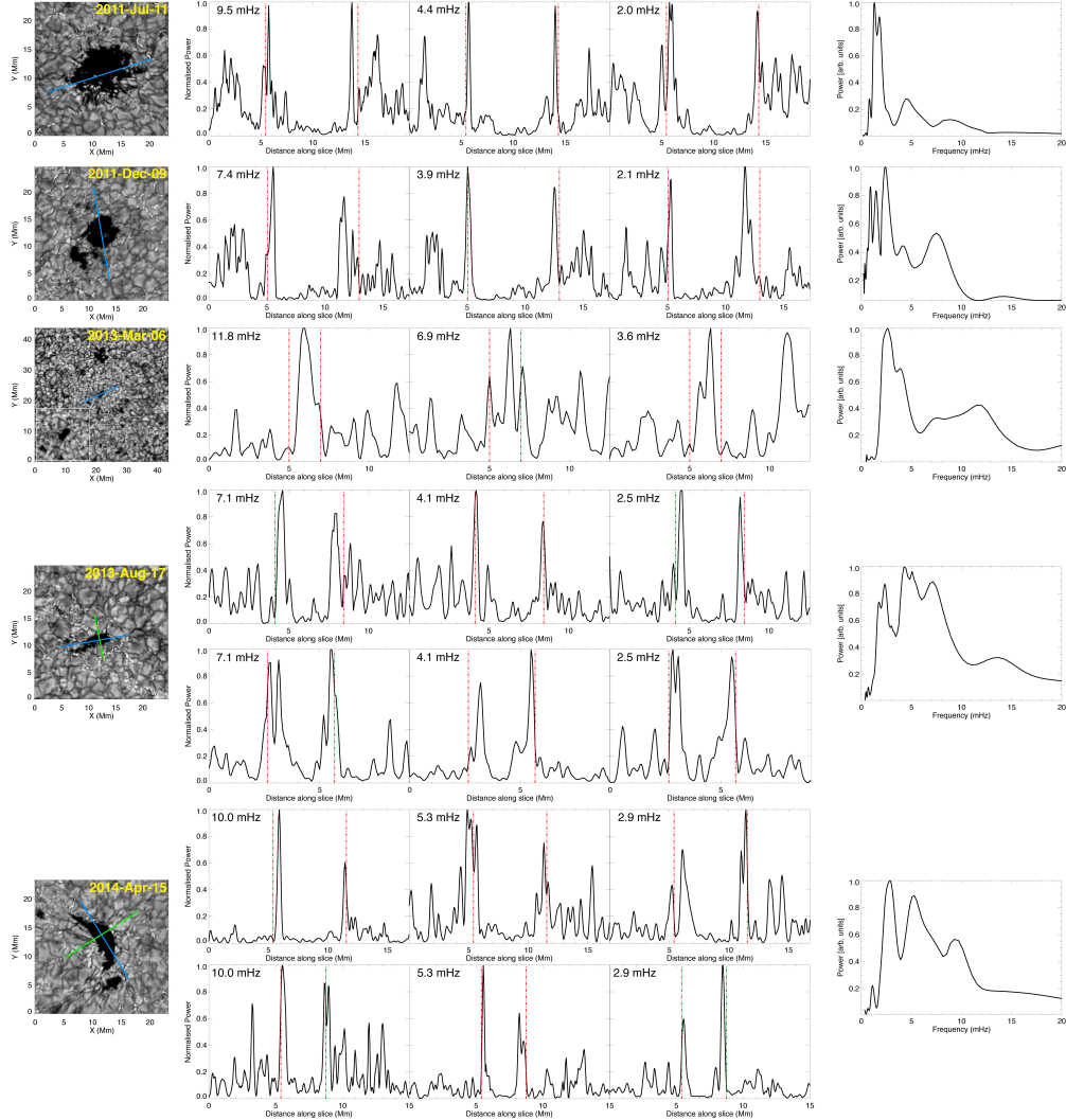
Figure 7. The left column displays a sample view of five further pores analysed for this study. All images are taken with the G-band filter ( 4305.5 \text{ \AA} ) with yellow labels in the upper right corners indicating the date of observation for the pore. A white box in the 2013-Mar-06 panel shows a 10 \text{ Mm} \times 10 \text{ Mm} zoom of the pore under investigation. Blue lines in these images indicate the cross-cuts used to plot the one-dimensional power cross-cuts shown in the plots on the right of each pore. The one-dimensional power cross-cuts for each pore is acquired at the specific dominant oscillation frequencies observed in the data, which have been isolated with a Gaussian filter. In the top left of each cross-cut the labels indicate the central frequency employed in the filter, while the red dashed lines indicate the pore boundary. Peaks at the boundary with a minimum in the center of the pore are a typical feature of the surface mode, while peaks in the center which decay to minima at the boundaries are a characteristic of the body mode. The final two pore images have an additional green line, which indicates an additional set of power cross-cut plots that have been included for these datasets. These cross-cuts are perpendicular to those shown from the blue cross-cut. The upper plot panels to the right of the pores show the plots for the blue line while the lower panels show the plots for the green line. The bottom two pore examples are more elliptical in nature than the other pores and these additional plots have been included to show that the power distribution can be seen at various angles around the pore. The final plots on the far right for each dataset shows the power as a function of frequency for the pores. The highest power appears within \sim 2-5 \text{ mHz} , which would suggest that p -modes are responsible for exciting the waves.
