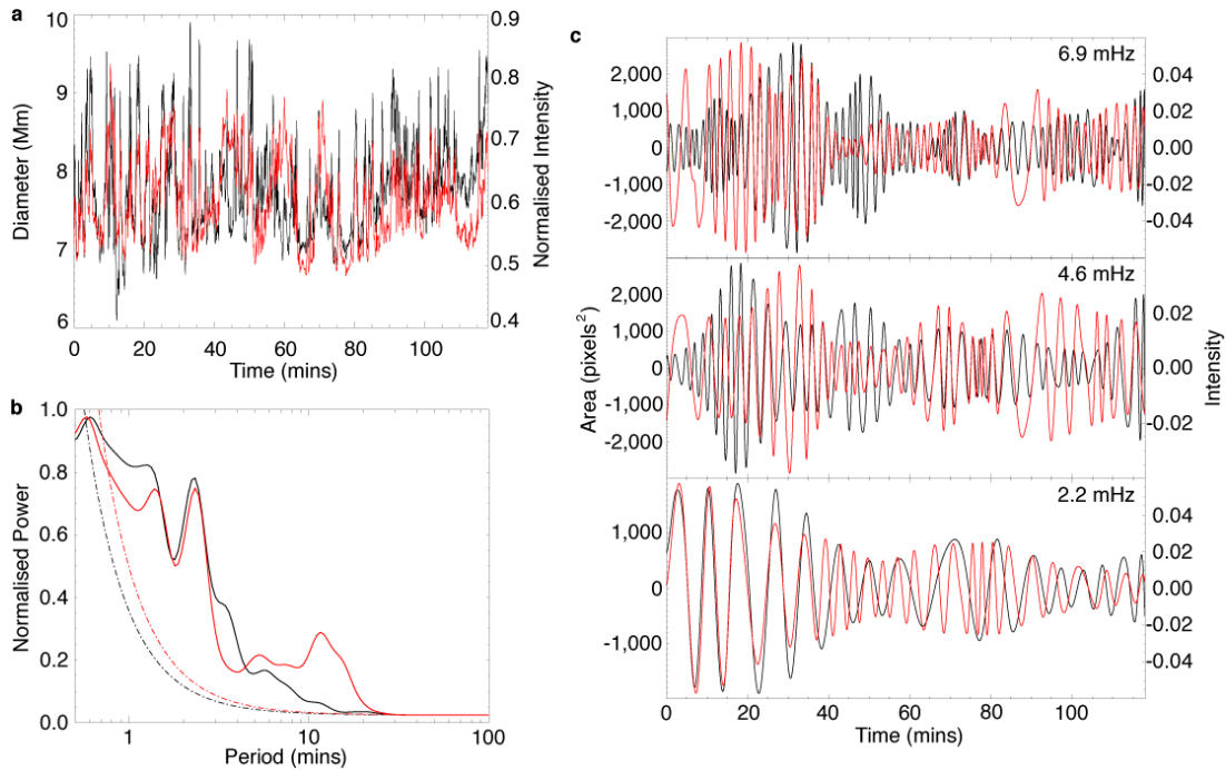
Figure 2. Multiple techniques are employed to determine oscillatory signals present in our data before filtering to observe the spatial distribution of the power. Panel a is the area ( black ) and intensity ( red ) signals established for a single pore over the duration of the observation sequence (2011 December 10 dataset). Panel b shows the dominant periods as determined by employing wavelet analysis on both the area and intensity signals with the dashed lines indicating the 99% significance levels. Panel c shows the result of employing the complementary empirical mode decomposition (EMD) technique on the area and intensity signals in a . Intrinsic Mode Functions (IMFs) at three different frequencies for both the area and intensity oscillations are displayed. This information is employed along with wavelet analysis to determine whether a sausage mode oscillation is present in the data, the dominant periods of oscillation and whether the fast/slow sausage mode is observed.
