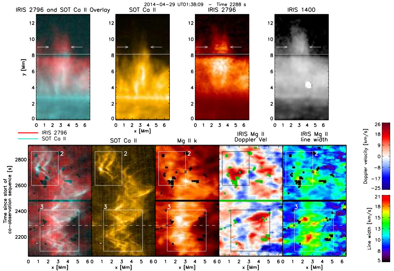
Figure 3. Hinode and IRIS observations of spicules. Similarly to Fig. 2 (case 1), we show here two other cases of spicule groups: one subject to a propagating kink wave (case 2), and another one subject to a rotation or a torsional Alfvén wave (case 3). See also the accompanying animation for this figure.
