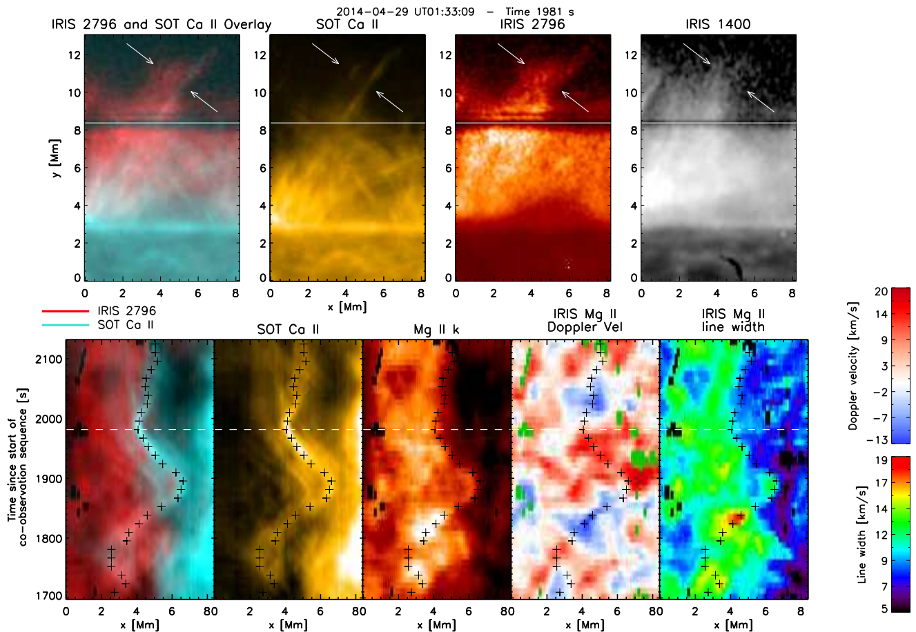
Figure 2. Hinode and IRIS observations of spicules. top panels: From left to right, composite image of IRIS SJI 2796 (red) & SOT Ca II H line (turquoise), the corresponding SOT image in the Ca II H line (yellow), the SJI 2796 image (red) and the SJI 1400 image (grey). In these images a spicule group is observed (marked within arrows). bottom panels: from left to right, time-distance diagrams at the IRIS slit location (horizontal white line on top panels) for the composite intensities of IRIS SJI 2796 (red) & SOT Ca II H line (turquoise), the SOT Ca II H line intensity (yellow), the SJI 2796 intensity (red), the Doppler velocity and line width in Mg II k. For the SOT intensity diagram we have summed over several cuts perpendicular to the oscillating structure, along 2 Mm length from the location of the IRIS slit crossing and above. The black crosses denote locations of maximum Ca II intensity within the spicule group. Green/black pixels in the Doppler/line width maps denote regions too dim to retrieve a quality fit. See also the accompanying animation for this figure.
