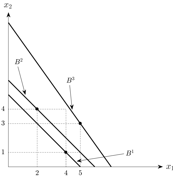
Figure 1: Violation of Additive Separability
