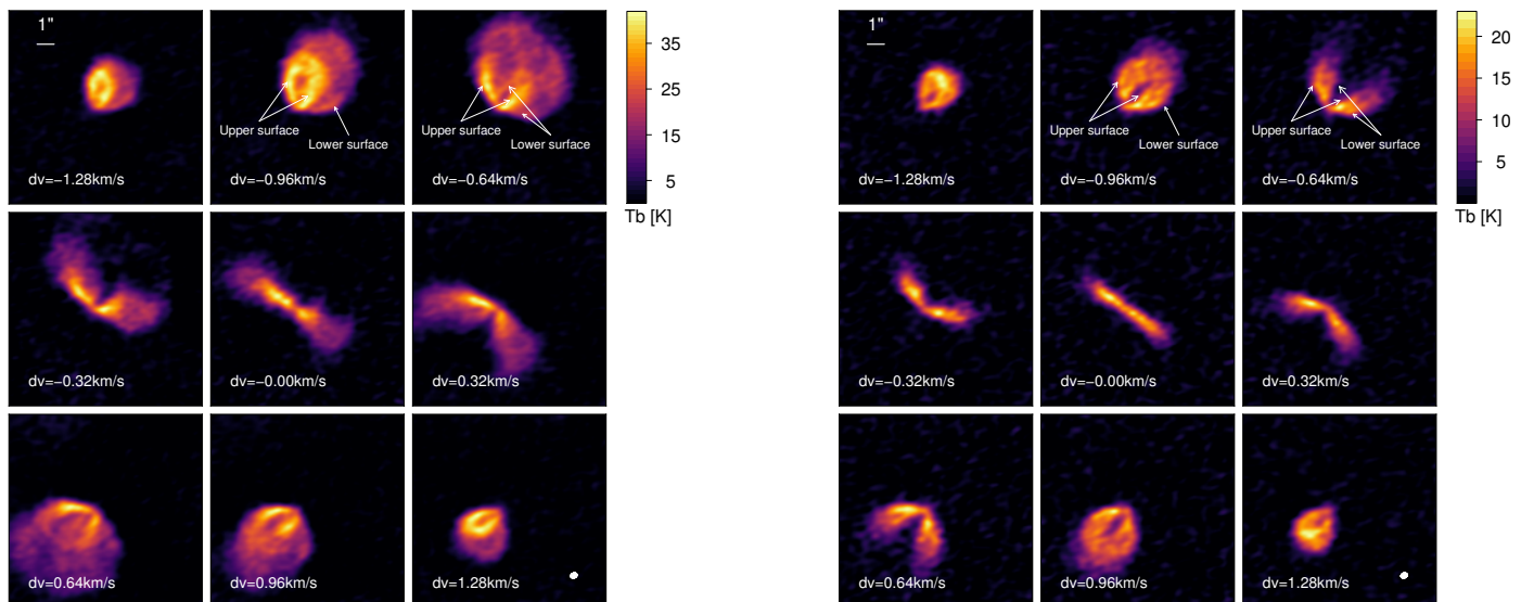
Fig. 1. Channel maps of ^{12}\text{CO} (left) and ^{13}\text{CO} (right) displayed with a channel width of 80 m/s. The data is not continuum subtracted. The dv is relative to the systemic velocity of 4.5 \text{ km.s}^{-1} . The beam is indicated in the bottom right corner.
