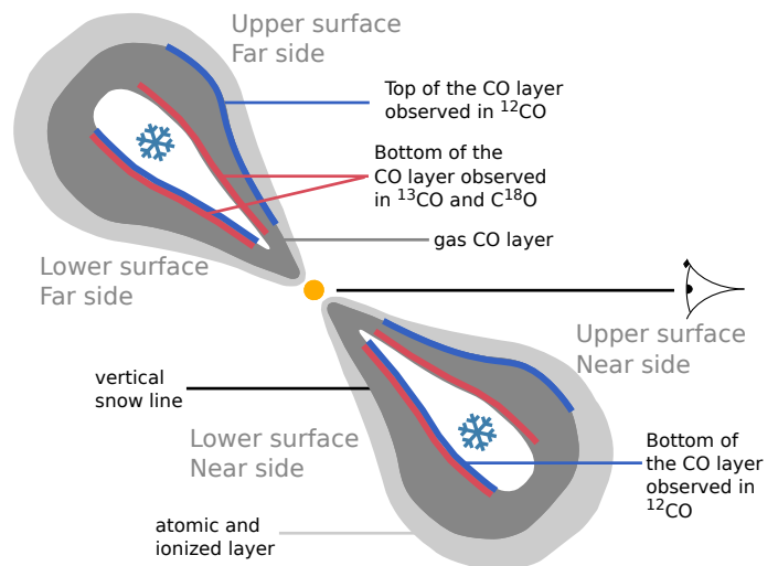
Fig. 3. Schematic view of the various layers observed in the CO lines.
