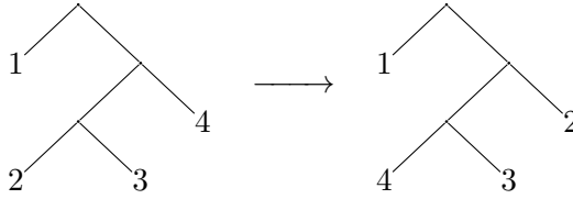
Figure 4: The map t_{100,11} denoted using tree-pairs
