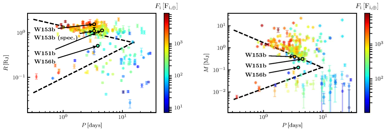
Fig. 10. WASP-151b, WASP-153b and WASP-156b in the radius versus orbital period (left) and the mass versus orbital period (right) domains. The colored points correspond to the known exoplanet and the color reflect their bolometric incident flux. WASP-151b, WASP-153b and WASP-156b are circled in black and the black dashed lines correspond to the upper and lower boundaries of the Neptunian desert as reported by (Mazeh et al. 2016). See Section 4.4 for details.
