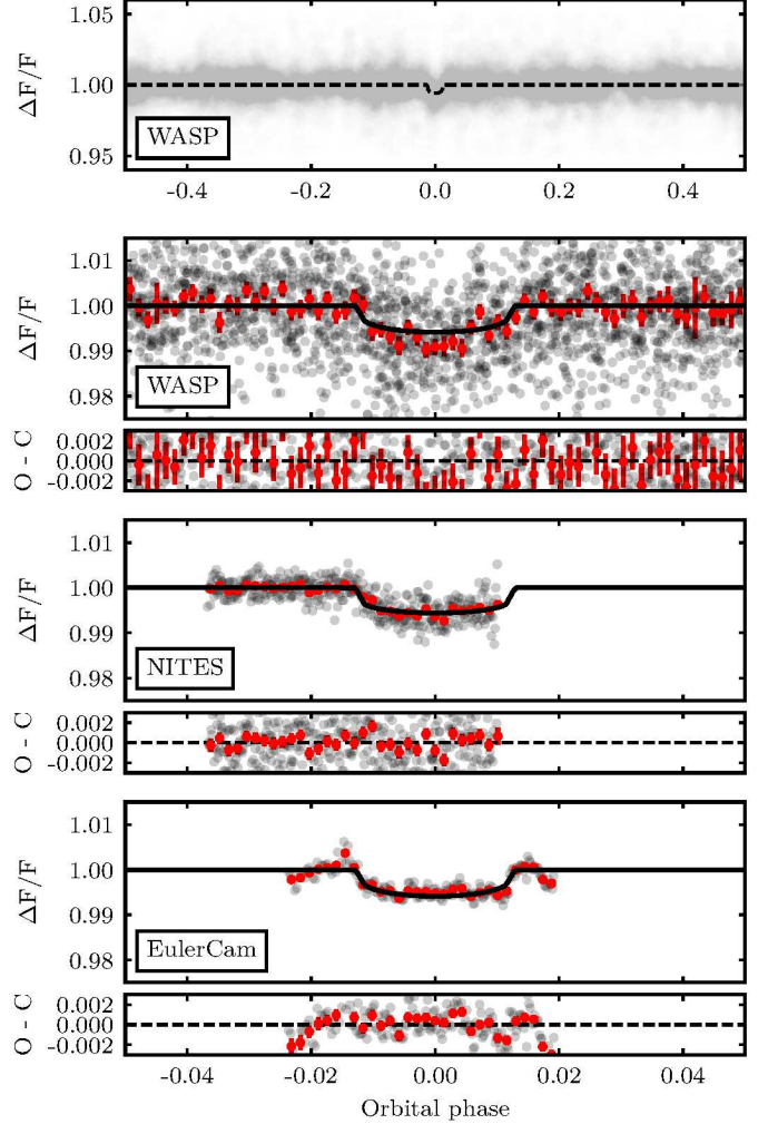
Fig. 6. Photometry of WASP-156. The black/grey points are the data points at the original cadence of the observations, displayed without error bars for clarity. The red points corresponds to the same data points binned in phase with a bin width equivalent to 8 minutes. These points are represented with their associated 1\sigma error bars. The black dashed and solid lines correspond to the best-fit model at the original and binned cadence respectively.
