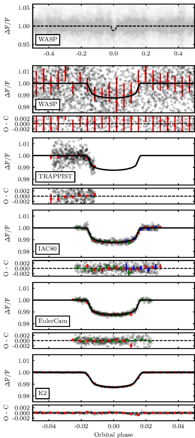
Fig. 2. Photometry of WASP-151. The black/grey points are the data points at the original cadence of the observations, displayed without error bars for clarity. The red points corresponds to the same data points binned in phase with a bin width equivalent to 29.424 minutes (Kepler long cadence). These points are represented with their associated 1\sigma error bars. The black dashed and solid lines correspond to the best-fit model at the original and binned cadence respectively. When several datasets have been gathered with the same instrument, they are displayed on the same figure but with different symbols and colors. September EulerCam and IAC80 data are red dots, October EulerCam and first part of the November IAC80 data are green pentagons, and second part of the November IAC80 data are blue triangles.
