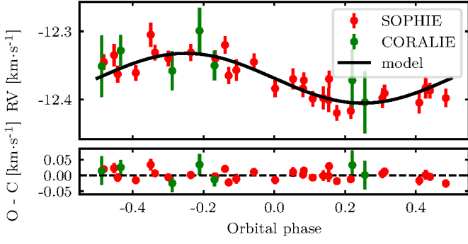
Fig. 3. Radial velocities of WASP-151. The data points are represented with their associated 1\sigma error bars.
