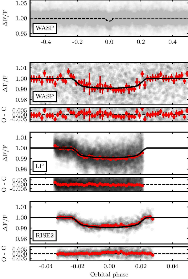
Fig. 4. Photometry of WASP-153. The black/grey points are the data points at the original cadence of the observations, displayed without error bars for clarity. The red points corresponds to the same data points binned in phase with a bin width equivalent to 8 minutes. These points are represented with their associated 1\sigma error bars. The black dashed and solid lines correspond to the best-fit model at the original and binned cadence respectively.
