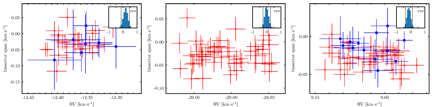
Fig. 1. Bisector span as a function of the radial velocities with 1\text{-}\sigma error bars for WASP-151, 153 and 156 (from left to right). SOPHIE data are the red circles; CORALIE data are the blue squares. The ranges here have the same extents in the x - and y -axes. For each star, the posterior probability function of the correlation coefficient is displayed in an insert located in the upper left corner.
