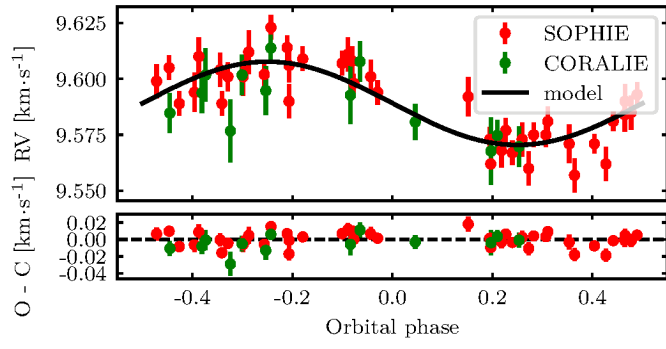
Fig. 7. Radial velocities of WASP-156. The data points are represented with their associated 1\sigma error bars.
