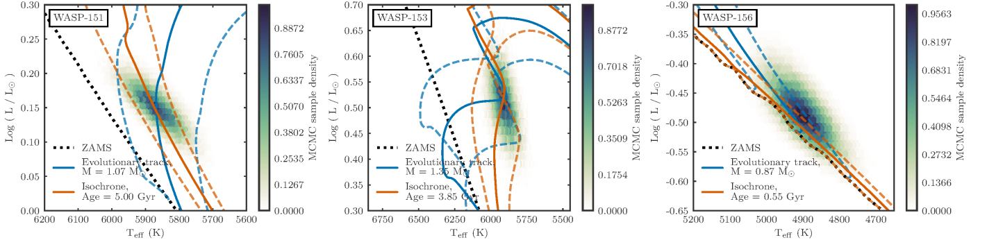
Fig. 8. WASP-151, WASP-153 and WASP-156 marginalized posterior distribution in the Hertzsprung–Russell diagram. The dotted black line correspond to the zero-age main sequence (ZAMS) at best-fit [\text{Fe}/\text{H}] . It's defined as the time at which the star reaches its minimum luminosity and stellar ages are measured relative to this time. The blue lines are stellar mass evolutionary tracks and the orange ones are age isochrones. For both isochrones and evolutionary tracks the solid line correspond to the best-fit model (maximum of joint likelihood distribution) and the dashed lines correspond to the two extrema of the 68 % confidence interval. For more details see Section 3.2.2 and Table A.5.
