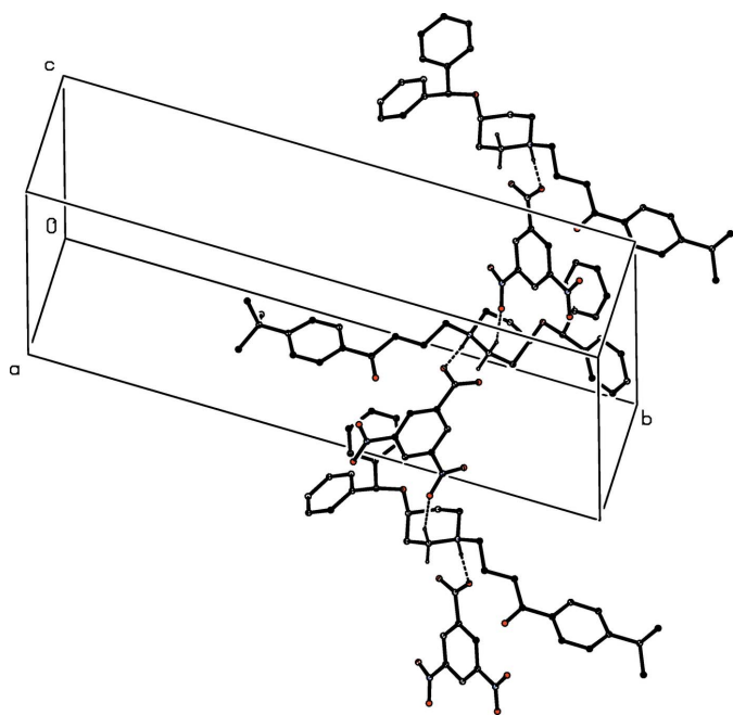
Figure 3 Part of the crystal structure of compound (I), showing a hydrogen-bonded C_2^2(11) chain running parallel to [20\bar{1}] . For clarity, the minor disorder component of the cation, and the H atoms bonded to C atoms not involved in the motif shown have been omitted.
