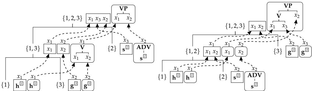
Figure 16 (Left) The only derivation tree of the LCFRS/sDCP hybrid grammar induced in Example 19 with the recursive partitioning extracted from the hybrid tree. (Right) The only derivation tree of the LCFRS/sDCP hybrid grammar induced in Example 20 with the left-branching recursive partitioning.
