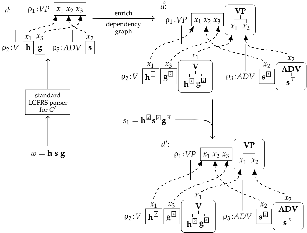
Figure 9 Algorithm 1 applied to the LCFRS/sDCP hybrid grammar G from Example 11 and the sentence w = \mathbf{h s g} .
