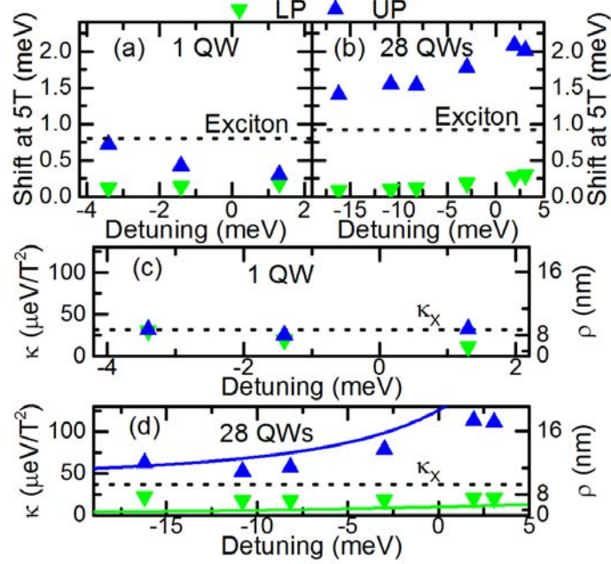
Fig. 4: Diamagnetic shifts of LP and UP at 5T for (a) the 1 QW-sample and (b) the 28 QW-sample as a function of detuning. The shift of the UP of the 28 QW-sample exceeds the bare exciton diamagnetic shift for all detunings. (c) Diamagnetic coefficients from fits according to Eq. (3) for the 1 QW-sample. (d) The same as (c) for the 28 QW-sample where \kappa_{UP} exceeds \kappa_X for all detunings. Solid lines are theoretical curves according to Eqs. (4) and (5) which yield \rho_{LP,UP} in the very strong coupling framework.
