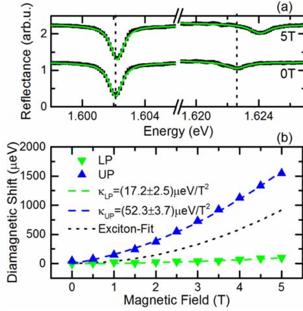
Fig. 3: (a) Reflectance spectra (black squares) at 0T and 5T for the 28 QW-sample at -10.8\text{meV} detuning. Green solid line shows the fit with two Lorentzian functions. Vertical dotted lines are the fitted polariton energies at zero magnetic field. (b) Diamagnetic shifts as a function of magnetic field. Dashed lines are fits according to Eq. (3) with \kappa as fitting parameter. Black dotted line is the fit to the bare exciton shift measured on a different piece of the same wafer.
