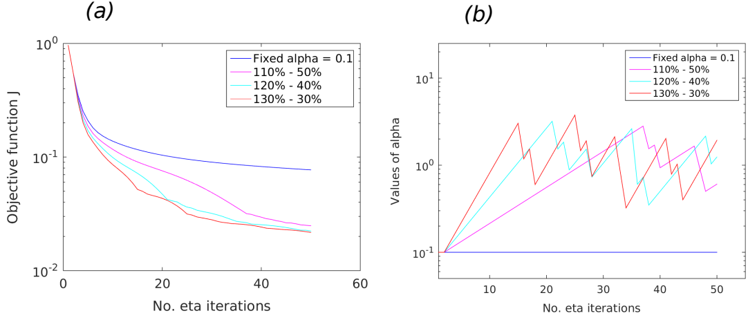
Figure 7: A semi-log plot shows the reductions of the objective functional J from using constant and adaptive \alpha s in (a). A semi-log plot shows the changes in the values of \alpha in (b). The colour version of this figure is online.
