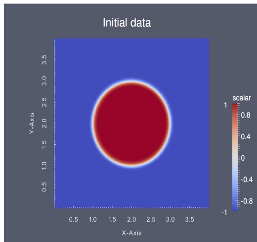
Figure 11: (a) shows the initial data from (4.1) and (b) illustrates the desired data from (4.6). The colour version of this figure is online.
