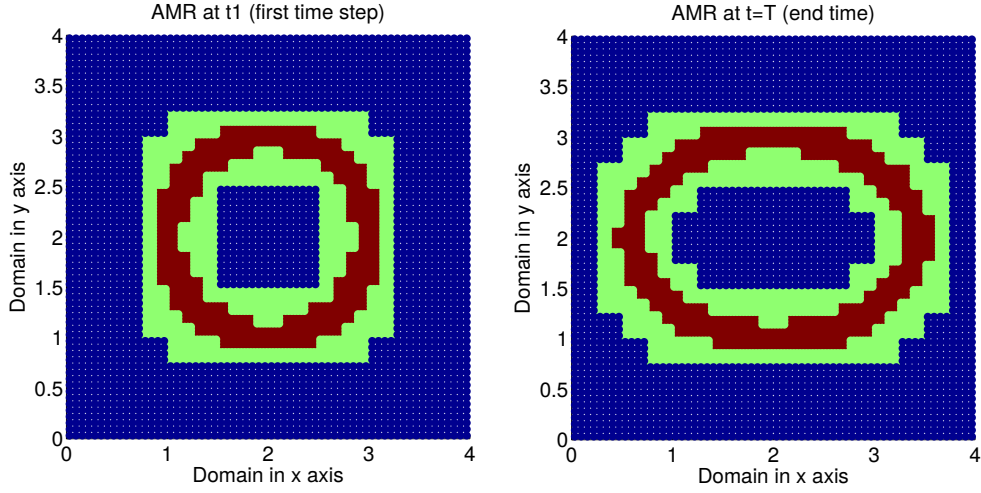
Figure 8: Two colour plots show the dynamic AMR in our solver. The blue region shows the 64^4 grid; light green region indicates the 128^2 grid; and finally red region illustrates the finest 256^2 grid. The colour version of this figure is online.
