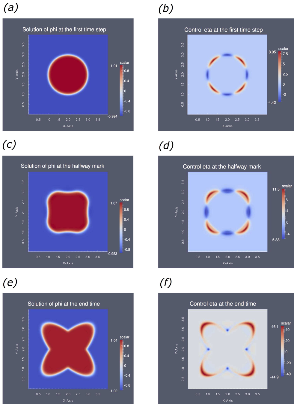
Figure 12: (a) and (b) show the solutions of \phi and \eta at the first time step, respectively; (c) and (d) illustrate the solutions at the halfway mark (i.e. t = 0.0025 ); (e) and (f) show the solutions at the final time T . The colour version of this figure is online.
