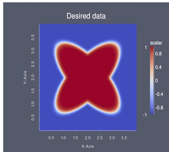
Figure 11: (a) shows the initial data from (4.1) and (b) illustrates the desired data from (4.6). The colour version of this figure is online.
