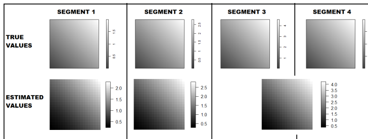
Figure 2: Simulated intensity functions for four time segments, with three change points (top panels) - Estimated segment intensities under the detection of two change points (bottom panels)
