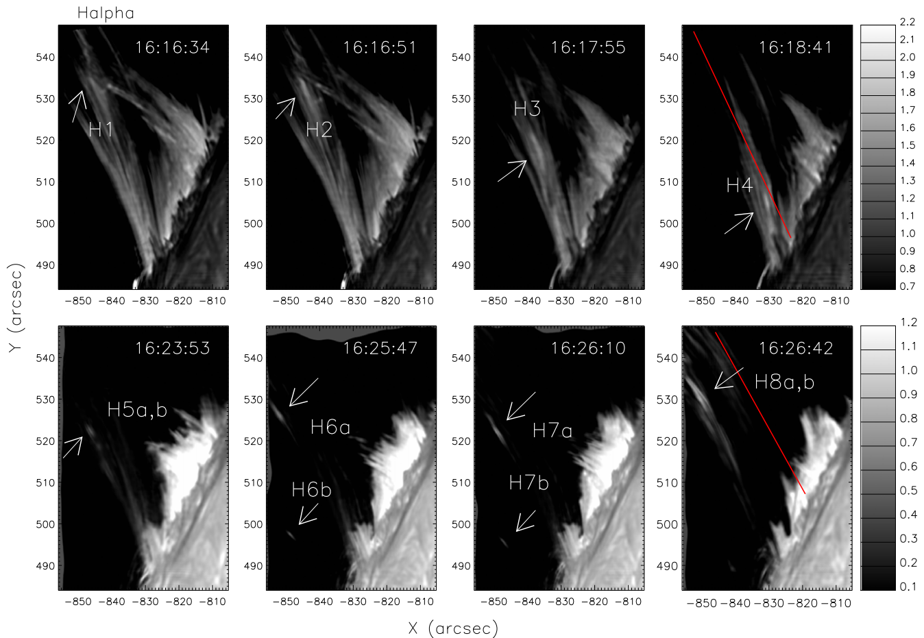
Figure 1. HARDcam H\alpha images from 2012 February 11 showing blobs of material falling back toward the solar surface (see the text). The top panel shows selected images for the first image sequence starting at 16:11:24 UT (series 1) and the lower panel shows selected images from the second sequence starting at 16:21:42 UT (series 2). Features of selected blobs can be found in Table 1. The lower right panels for each H\alpha sequence also shows the trace for the X–T cuts used in Figure 6.
