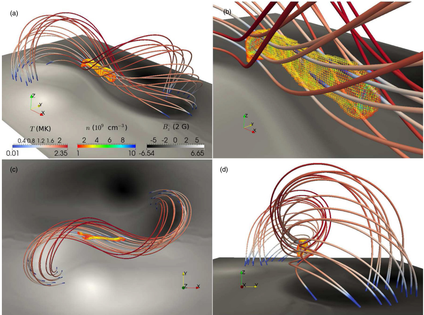
Figure 2. FR with embedded prominence at t = 150 minutes. Shown are field lines colored by temperature in blue to red, the prominence colored by density in a rainbow of colors, and the bottom magnetogram in gray. Panels (a), (c), and (d) are the side, top, and axial views, respectively. Panel (b) zooms in on (a). View (c) shows the filament spine within the S-shaped FR with the barb near its left end.
