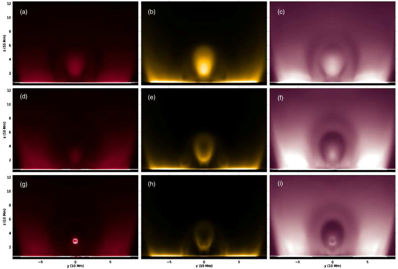
Figure 3. Synthetic SDO/AIA views showing the condensation process. We view along the x axis at times 11.4, 17.2, and 21.5 minutes from top to bottom, respectively. Approximate wavelength and peak temperature sensitivity are from left to right: 304 Å (0.08 MK), 171 Å (0.8 MK), and 211 Å (1.8 MK). (A color version of this figure is available in the online journal.)
