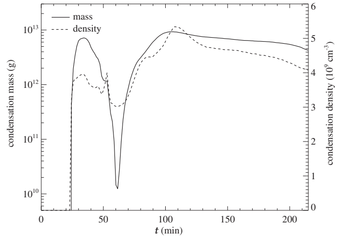
Figure 1. Evolution of the total mass (solid) and average number density (dashed) of the prominence.
