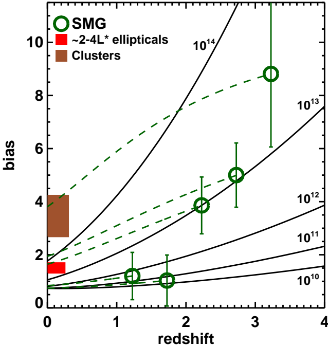
Figure 5. Predicted galaxy bias evolution of SMGs (open green circles) at z > 1 , plotted against redshift. The solid black lines represent the expected bias evolution for dark matter halos with constant masses (labelled, in solar masses). We trace the mass growth of halos hosting SMGs in green dashed lines, using the formalism from Fakhouri et al. (2010). We also plot typical bias measurements of \sim 2-4L^* galaxies (from the luminosity-bias relation derived in Zehavi et al. 2011) and optically selected galaxy clusters at redshifts 0.1 < z < 0.3 (Estrada et al. 2009).
