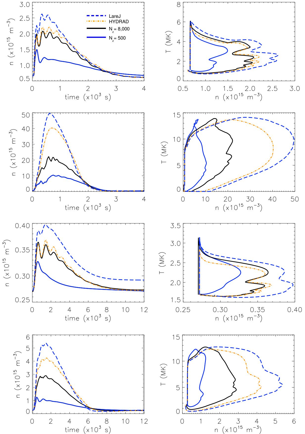
Fig. 9. Results for Cases 2 ( upper two panels ), 6 ( upper central two panels ), 8 ( lower central two panels ) and 12 ( lower two panels ). The panels show the coronal averaged density as a function of time and the temperature versus density phase space plot.
