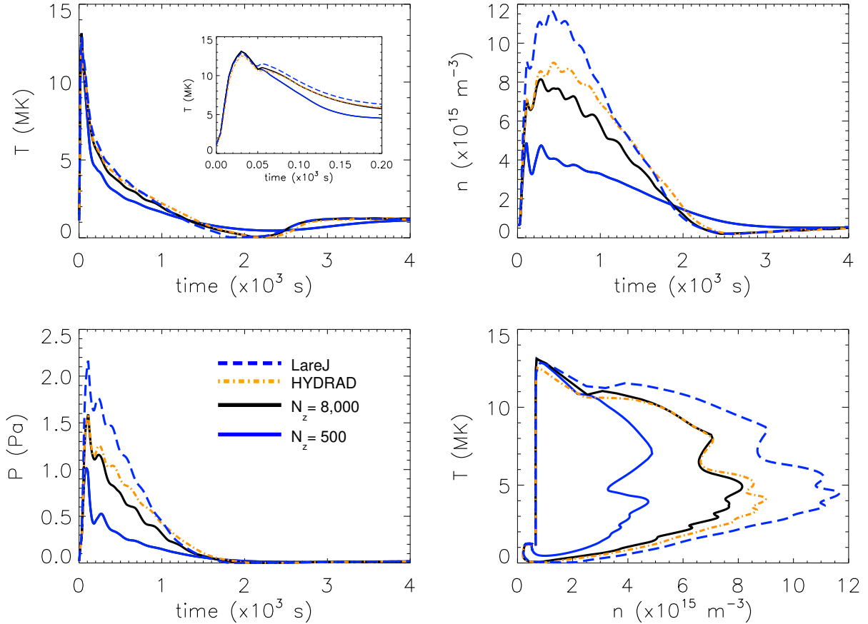
Fig. 7. Results for Case 3. Notation is the same as Fig. 4 but note the different time axis.
