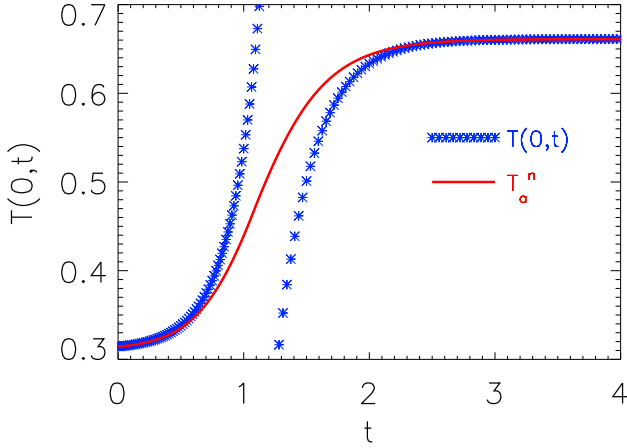
Fig. B.1. Temporal evolution of T(0, t) . The solution leaves a thermally unstable isothermal equilibrium and approaches a new stable, non-isothermal equilibrium. The solid red curve is the numerical solution obtained by using the RKL2 STS method ( T_a^n ) and the blue asterisks represent the corresponding linear solutions ( T(0, t) ). The units on both axes are arbitrary.
