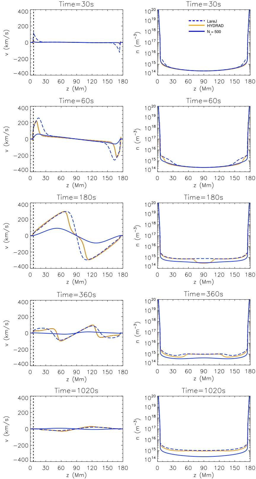
Fig. 6. Results for Case 9. The panels show the velocity and density as functions of position for times during the evaporation phase up until the second density peak. The dashed blue line is the LareJ solution (that is computed with 500 grid points along the length of the loop), the solid blue line is the Lare1D solution that is computed with 500 grid points along the length of the loop and the solid orange line corresponds to the HYDRAD solution. The dashed black line indicates the position of the top of the UTR ( z_0 ).
