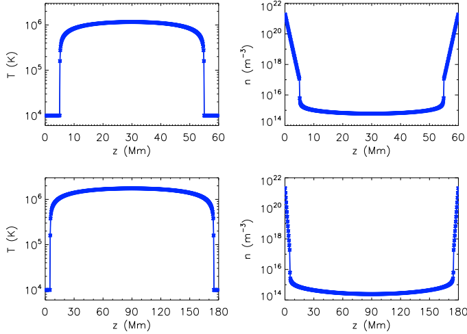
Fig. 1. Temperature and density initial conditions with 500 grid points along the length of the loop. Upper panels: 60 Mm loop with Q_{\text{bg}} = 2.2167 \times 10^{-5} \text{ J m}^{-3} \text{ s}^{-1} . Lower panels: 180 Mm loop with Q_{\text{bg}} = 6.8682 \times 10^{-6} \text{ J m}^{-3} \text{ s}^{-1} . Each asterisk represents a single grid point.
