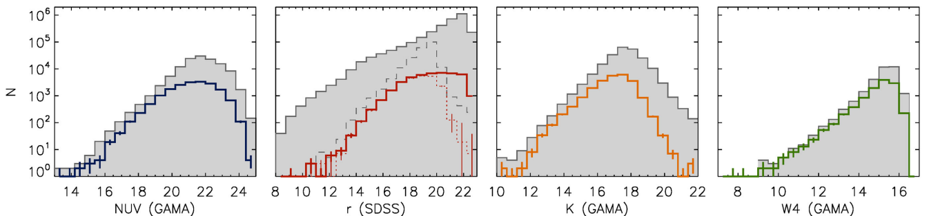
Figure 15. Histograms (solid coloured lines) of the magnitudes of reliable H-ATLAS IDs in NUV, r , K and W4 ( 22\text{-}\mu\text{m} ). The background distributions in each band are shown by the filled histogram. The r -band histogram contains all SDSS objects in the optical catalogue (including stars, galaxies and quasars). The dashed grey line shows the distribution of r -band magnitudes in the GAMA galaxy sample. For comparison, we show the magnitude distribution of all reliable IDs in SDSS (solid red line), and that of IDs in GAMA (dotted red line). Photometry in the other bands is drawn from the GAMA photometric catalogue only.
