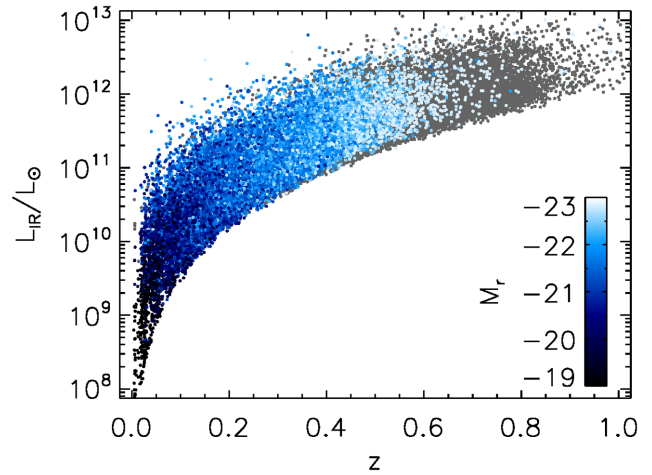
Figure 19. Total IR luminosities of all reliable extragalactic H-ATLAS IDs as a function of redshift. Luminosities were estimated by fitting the 100\text{--}500 \mu\text{m} fluxes with a modified blackbody SED with fixed \beta = 1.82 and free temperature and normalization, and applying a correction factor of 1.35 as described in the text. For the subset of IDs in GAMA, we colour the data by the r -band absolute magnitude measured from KCORRECT.
