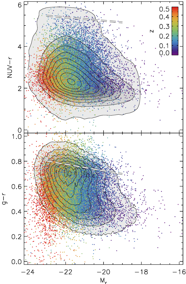
Figure 16. Rest-frame colour–magnitude diagrams in \text{NUV} - r and g - r for reliable IDs in GAMA, in comparison to the full GAMA sample (grey-scale contours). The thick dashed line in each panel shows the red sequence derived from the GAMA sample in Bourne et al. (2012). Note that H-ATLAS selects galaxies throughout the full locus of GAMA galaxies.
