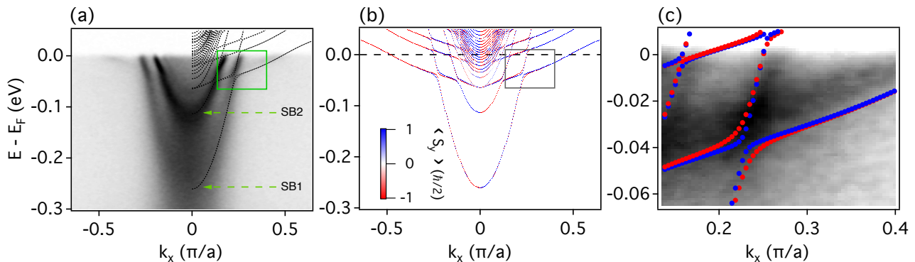
FIG. 1. (color online)(a) Subband structure of the STO (001) surface 2DEL from HR-ARPES (greyscale plot) taken at 47 eV with s -polarized light along the [100] direction. Note that throughout this paper all momenta are given relative to the \Gamma point of the second Brillouin zone at (k_x, k_y) = (2\pi/a, 0) . The result of self-consistent tight binding supercell calculations is over-plotted (black dashed lines).(b) Band structure calculation from (a) with color-coded spin expectation values \langle S_y \rangle .(c) Region of energy-momentum space indicated by the green box in (a), measured with p -polarized light at 47 eV to enhance the intensity of the heavy subband which has out-of-plane orbital character.
