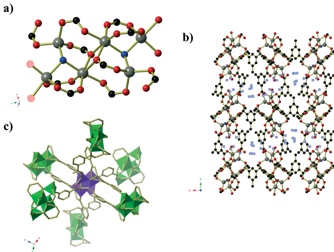
Fig. 2 a) The Zn 6 (OH) 2 (CO 2 ) 10 (H 2 O) 3 cluster found in Zn 6 (mip) 5 (OH) 2 (H 2 O) 4 ·xH 2 O (x ≈ 7.4, compound 2). The two μ 3 -OH anions are shown in blue, and major sites of the disordered coordinated water molecules are shown as hatched red circles. b) A view along the channels of the α-Po net of Zn 6 (mip) 5 (OH) 2 (H 2 O) 4 ·xH 2 O (x ≈ 7.4). Partial occupancy water molecules are shown as hatched blue spheres. Hydrogen atoms have been omitted for clarity. c) The connectivity of the Zn 6 (OH) 2 (CO 2 ) 10 (H 2 O) 3 clusters which act as six-connecting nodes in the α-Po net. The Zn centres belonging to the central and peripheral clusters are shown in purple and green, respectively. Terminal methyl groups, coordinated water molecules and monodentate carboxylate groups have been omitted for clarity.
