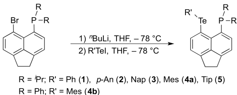
Scheme 1. Synthesis of peri -substituted P,Te systems.
