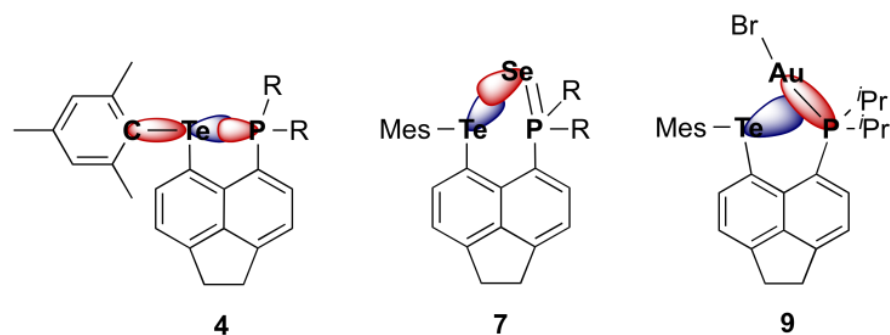
Figure 8. Proposed orbital interactions in the compounds 4 , 7 and 9 causing the transfer of spin information through space.
