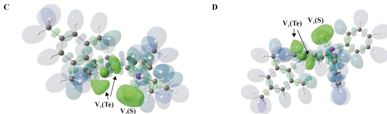
Figure 7. top: AIM bond paths of 6b (A) and 6a (B). Bond critical points are given as red dots and ring critical points are shown as yellow dots. All structures are AIM2000 representations. bottom: Isosurface representation of the localization domains of the ELI-D ( Y = 1.40 ) of 6a (C) and 6b (D), the lone-pair basins ( V_1 ) of Te and S are colored green. All remaining ELI-D basins are given in transparent mode for clarity reasons.
