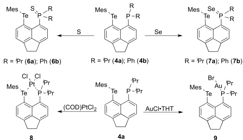
Scheme 2. Reactions of peri -substituted P,Te systems.
