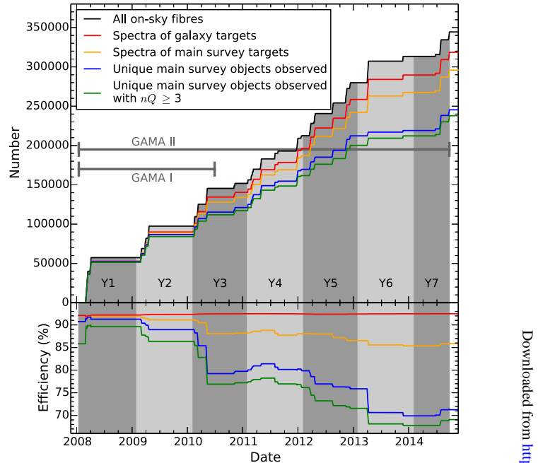
Figure 8. Evolution of the GAMA II spectroscopic survey on the AAT. The upper panel shows the progress of the survey in terms of the numbers of on-sky fibres, target spectra and unique objects observed, as indicated. The lower panel shows the average past survey efficiency, i.e. the numbers of the upper panel relative to the number of on-sky fibres. The colour coding is the same as in the upper panel. The temporary increase of the efficiency in 2010–2011 corresponds to the expansion of the survey from GAMA I to GAMA II (cf. Section 2.1).
