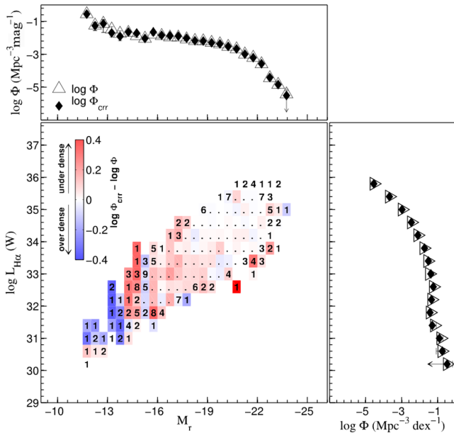
Figure 5. The residual map showing the difference in number densities derived using the classical ( \Phi ) and the density corrected ( \Phi_{\text{crr}} ) V_{\text{max}} methods for the z < 0.1 bivariate functions. The colours indicate the difference between \Phi_{\text{crr}} and \Phi . A positive difference (redder colours) implies that f_v corrects V_{\text{max}} for an overdensity and negative (bluer colours) means the correction is for an underdensity. Top and right-hand panels show the M_r and \text{H}\alpha univariate LFs.
