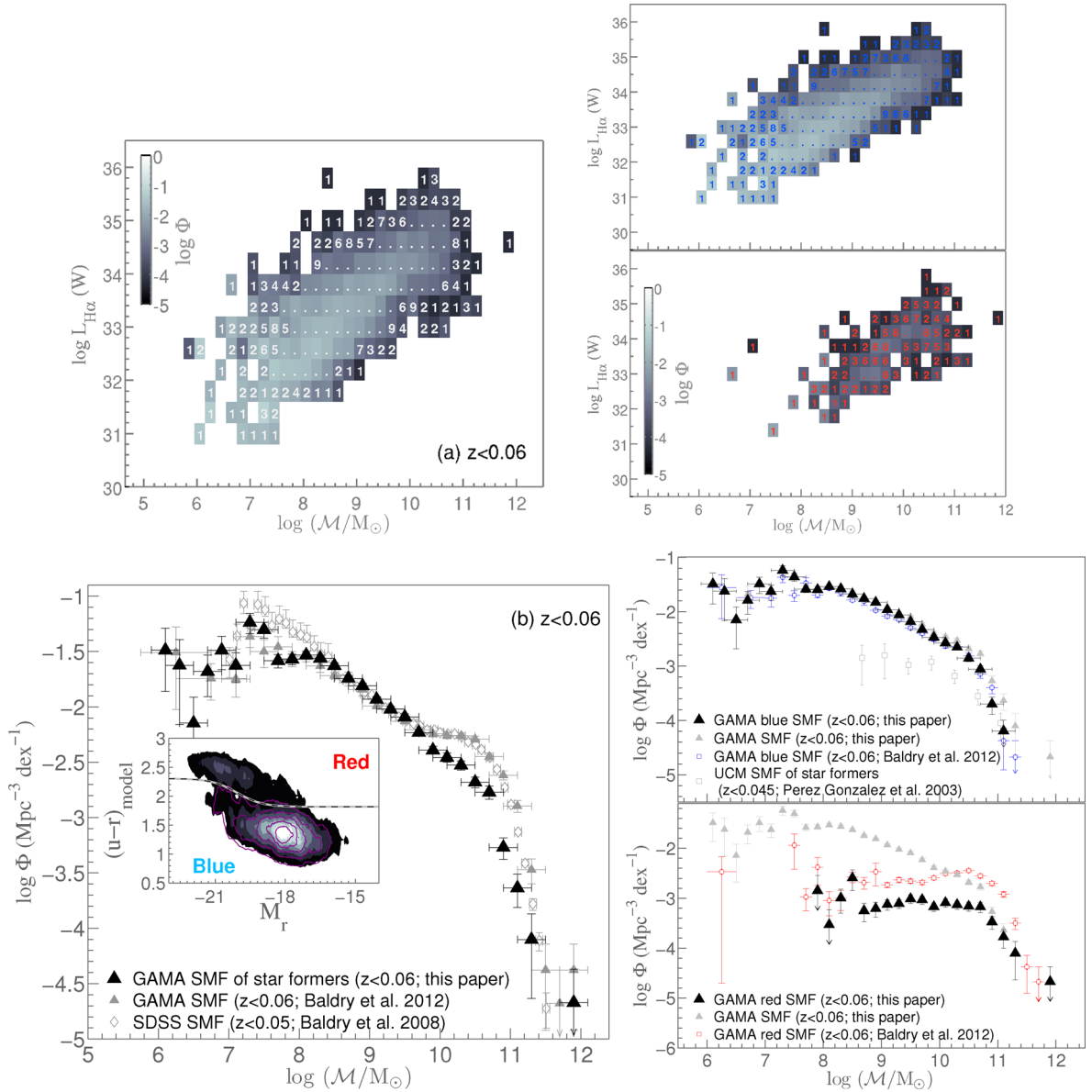
Figure 15. (a) The z < 0.06 GAMA bivariate L_{\text{H}\alpha}-\mathcal{M} functions of all, blue and red SF galaxies (left, top right and bottom right panel, respectively), constructed using the density corrected 1/V_{\text{max}} method described in Section 3.2. The grey-scale indicates the log of number densities ( \Phi ) in the unit of \text{Mpc}^{-3} \text{dex}^{-2} . (b) The SMFs obtained from integrating the bivariate L_{\text{H}\alpha}-\mathcal{M} functions over L_{\text{H}\alpha} are compared to the z < 0.06 GAMA SMFs of Baldry et al. (2012) and z < 0.05 SDSS SMF of Baldry, Glazebrook & Driver (2008).
