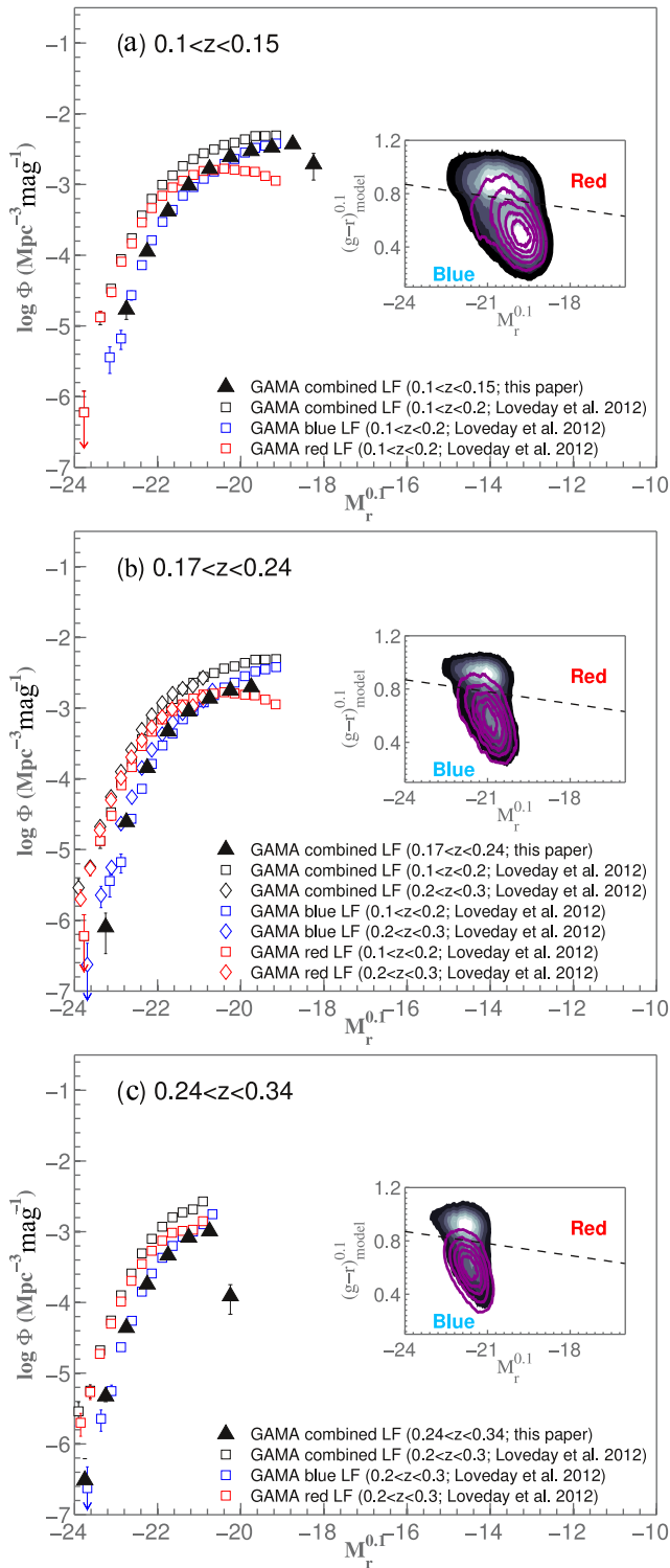
Figure 9. GAMA higher- z M_r^{0.1} LFs of all SF galaxies computed by integrating the bivariate L_{\text{H}\alpha} - M_r functions. The open symbols in each panel show the GAMA all, blue and red M_r^{0.1} LFs of Loveday et al. (2012) over similar redshift ranges. The insets show the data density distributions in (g-r)_{\text{model}}^{0.1} and M_r^{0.1} of all galaxies regardless of star formation (grey shading) and SF galaxies with F_{\text{H}\alpha} > 1 \times 10^{-18} \text{ W m}^{-2} (magenta contours). These distributions correspond to the redshift ranges given in the plot key. The colour-magnitude cut (equation 4) is shown as a dashed line.
