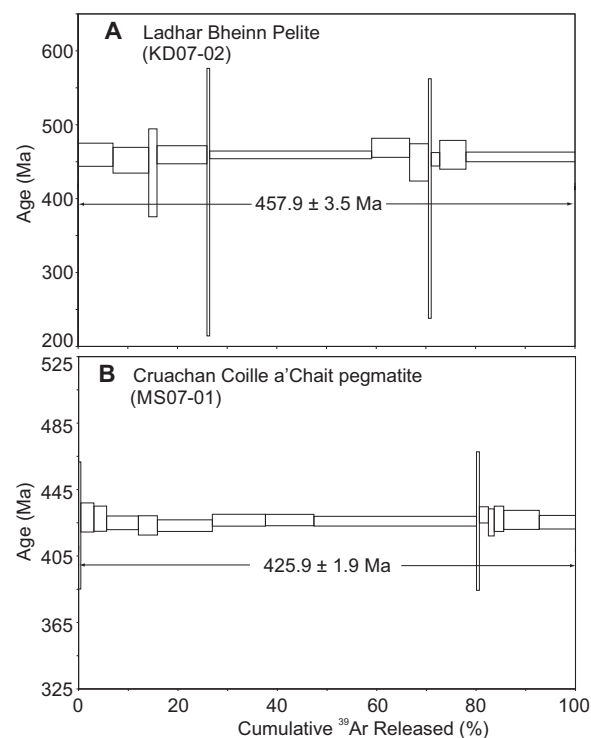
Figure 11. Argon data for Ladhar Bheinn Pelite (KD07-02) and Cruachan Coille a'Chait pegmatite (MS07-01).
