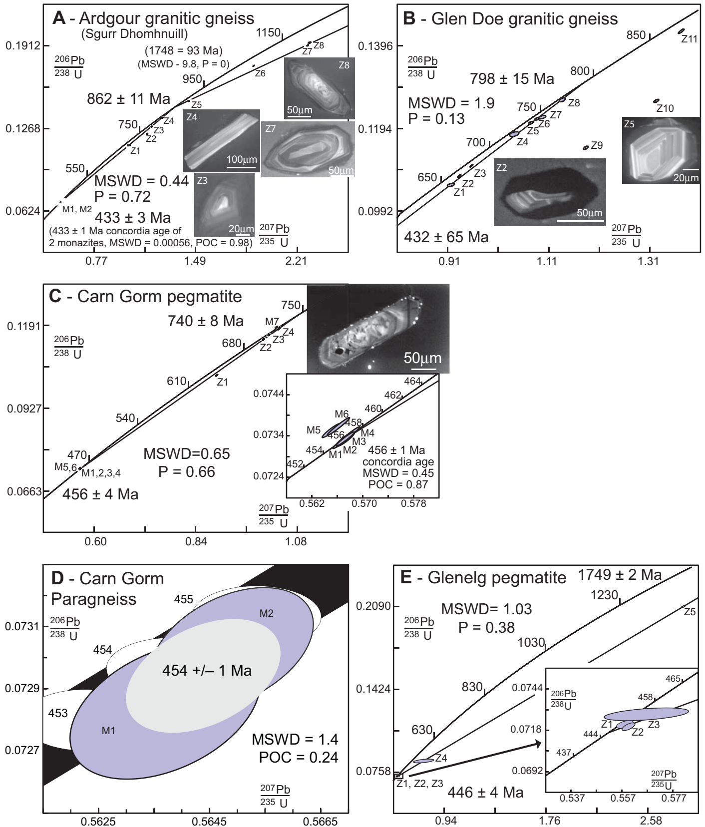
Figure 6. Concordia plots for thermal ionization mass spectrometry (TIMS) data from (A) Ardgour granitic gneiss (Sgurr Dhomhnuill), (B) Glen Doe granitic gneiss (sample SH-02-18B), (C) Carn Gorm pegmatite, (D) Carn Gorm paragneiss, (E) Glenelg pegmatite. P —probability of fit; POC—probability of concordance and equivalence; MSWD—mean square of weighted deviates.
