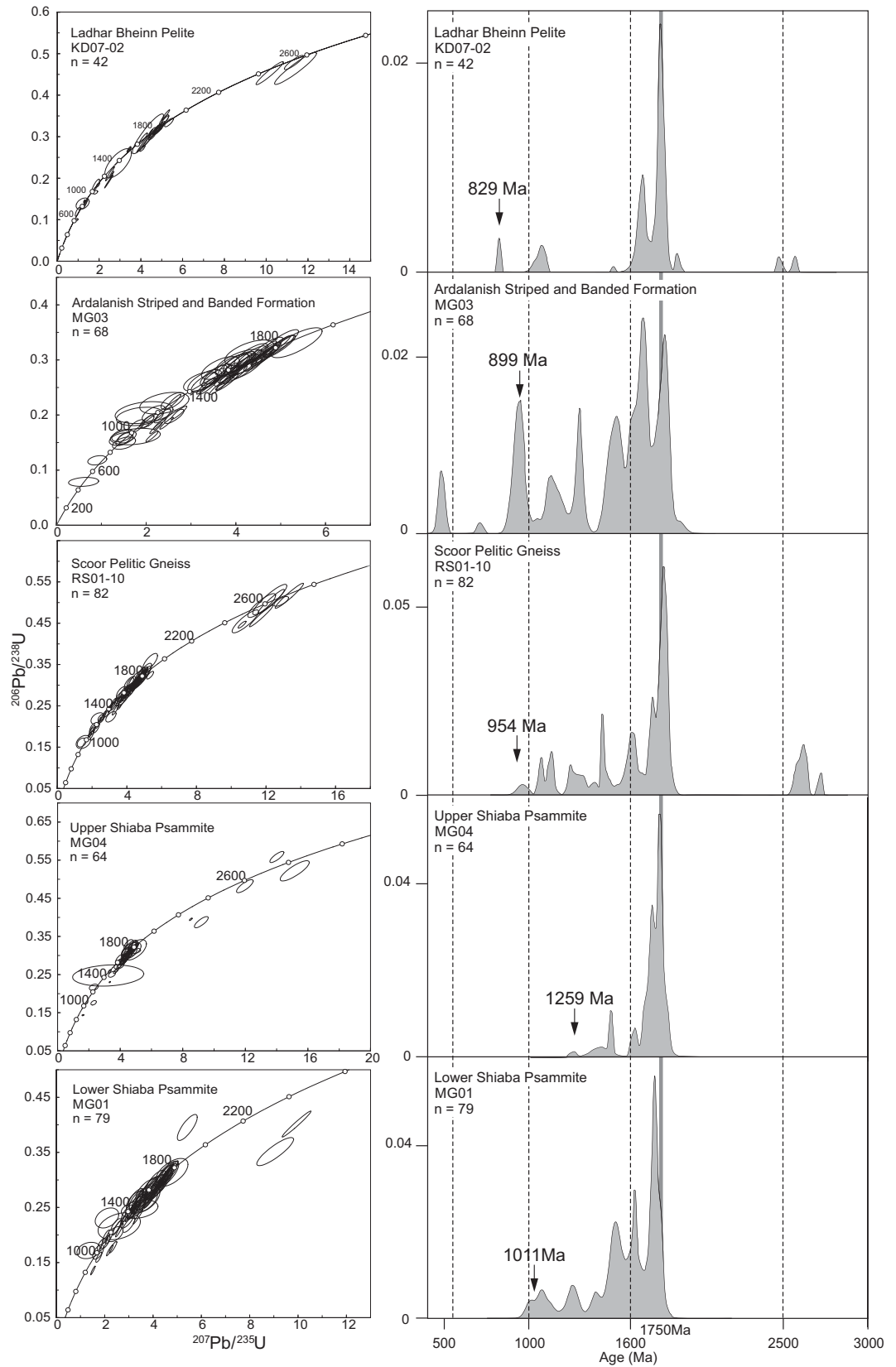
Figure 5. (Left column) Concordia diagrams based on ^{204}\text{Pb} -corrected zircon U-Pb data for samples of psammitic and pelitic rocks from the Ross of Mull and Knoydart. Error ellipses are shown at the 2\sigma level. Analytical data are available from the GSA Data Repository (see text footnote 1); n = number of zircon analyses in each sample. (Right column) Probability density distribution diagrams for detrital zircon data from psammitic and pelitic samples from the Ross of Mull and Knoydart. Dashed vertical lines separate boundaries of the Paleoproterozoic, Mesoproterozoic, and Neoproterozoic and are taken at 1600 Ma, 1000 Ma, and 545 Ma. Solid gray line highlights 1750 Ma age. The small arrows indicate the age of the youngest detrital zircon; n = number of zircon analyses in each sample. Analytical data are available from the GSA Data Repository (see text footnote 1).
