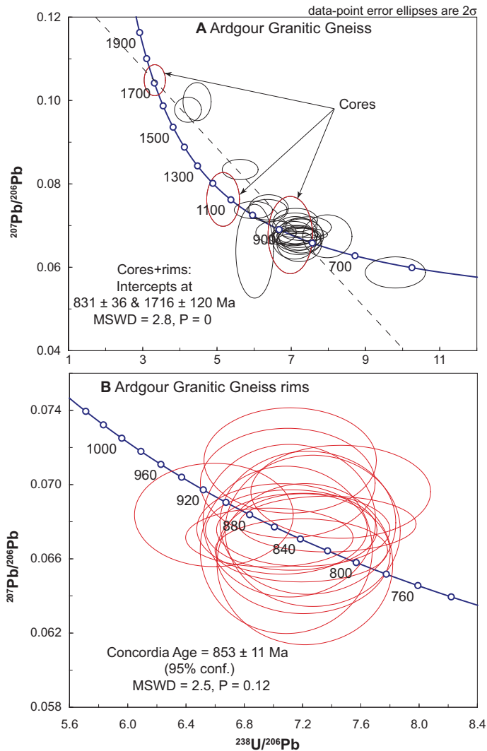
Figure 7. (A) Inverse concordia plot of secondary ion mass spectrometry (SIMS) data for Ardgour granitic gneiss. (B) Enlarged section of the concordia curve highlighting analyses of grain rims. P —probability of fit; MSWD—mean square of weighted deviates.
