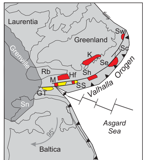
Figure 13. Neoproterozoic reconstruction of eastern Laurentia and Baltica prior to opening of Iapetus Ocean (adapted from Cawood et al., 2010). Baltica is shown in post-1000 Ma position with respect to Laurentia after it has undergone some 95° of clockwise rotation creating the Asgard Sea. Highlighted are the successions associated with the Valhalla orogen. Red blocks correspond to sedimentary and deformational sequences associated with Renlandian orogenic cycle of Valhalla orogen, and yellow blocks correspond to Knoydartian cycle. Abbreviations: GT—Grampian terrane (Badenoch Group); M—Moine succession; Hf—Hebridean foreland; K—Krummedal succession; Rb—Rockall Bank; SS—Svaerholt and Sørøy successions; Sh—Shetland Islands; Sn—Sveconorwegian orogen; Se—Eastern terrane of Svalbard; Sc—Central terrane of Svalbard; Sw—Western terrane of Svalbard.
