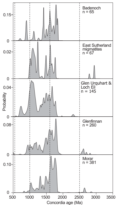
Figure 12. Probability plots comparing detrital zircon ages from lithostratigraphic units of the Moine Supergroup and correlatives within the sub-Grampian basement south of the Great Glen fault (Badenoch Group). Sources of data: Morar Group (this paper; Friend et al., 2003; Kirkland et al., 2008); Glenfinnan Group (this paper; Friend et al., 2003; Kirkland et al., 2008); Loch Eil Group and Glen Urquhart succession (Cawood et al., 2004); East Sutherland migmatites (Friend et al., 2003; as modified by Cawood et al., 2004); and Badenoch Group (Cawood et al., 2003).
