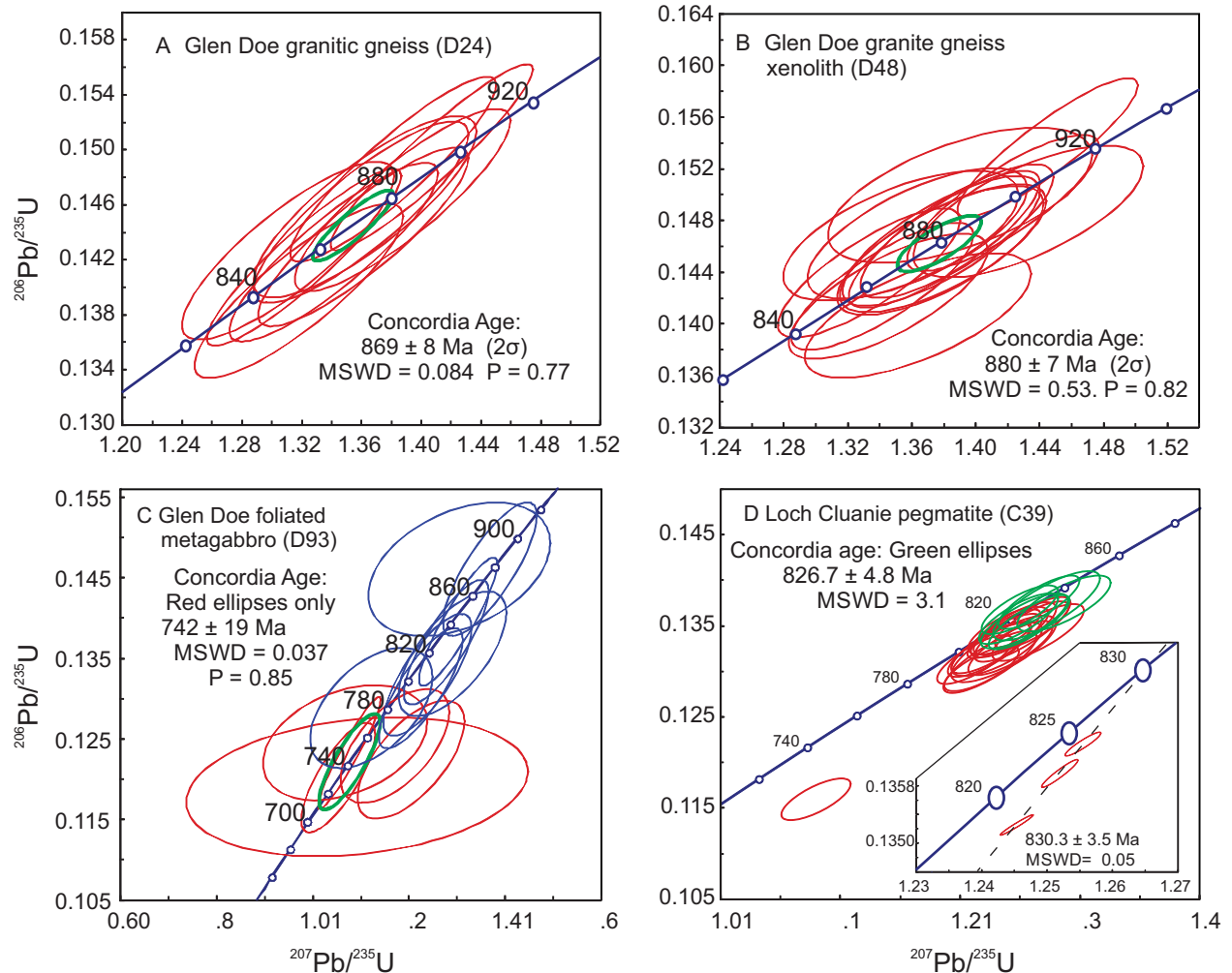
Figure 9. Data for Glen Doe granitic gneisses and metagabbro, and Loch Cluanie pegmatite: (A) concordia plot of granite gneiss sample D24, (B) concordia plot of granite gneiss sample D48, (C) concordia plot of foliated metagabbro sample D93, and (D) concordia plot of Loch Cluanie pegmatite sample C39. Analyses of Glen Doe zircons were undertaken by secondary ion mass spectrometry (SIMS), whereas Loch Cluanie zircons were analyzed by inductively coupled plasma–mass spectrometry (ICP-MS; main diagram) and thermal ionization mass spectrometry (TIMS; inset). Error ellipses are shown at 2\sigma level. P —probability of fit; MSWD—mean square of weighted deviates.
