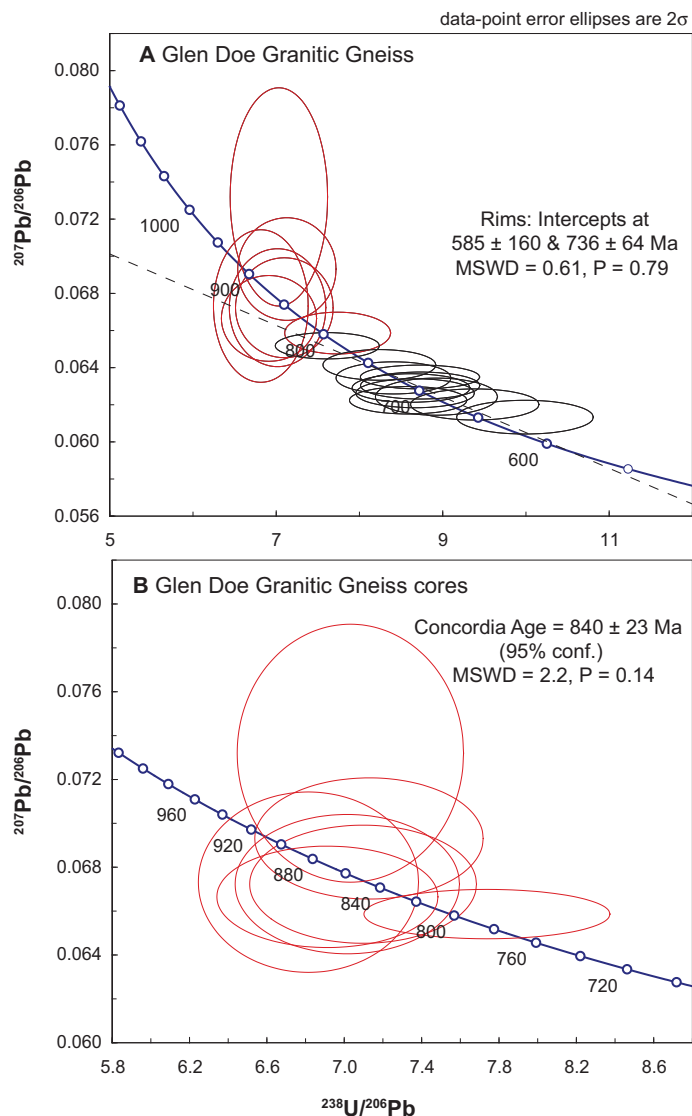
Figure 8. Inverse concordia plot of secondary ion mass spectrometry (SIMS) data for the Glen Doe granitic gneiss (SH-02–18B). (B) Enlarged section of the concordia curve showing analyses from grain cores.
