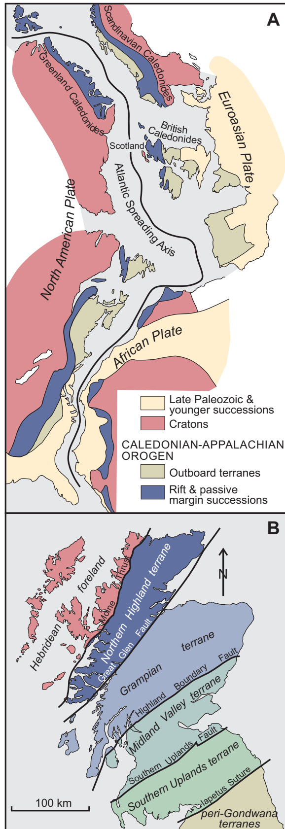
Figure 1. (A) Pangean reconstruction of North America, Europe, and Africa prior to opening of Atlantic (adapted from Williams, 1984). (B) Principal tectonostratigraphic units of northern England and Scotland.
