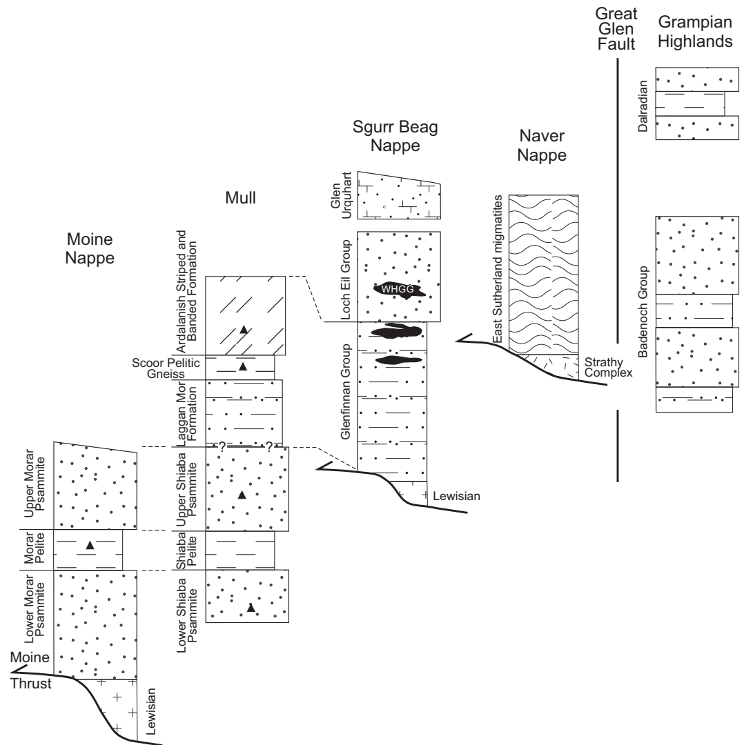
Figure 3. Schematic stratigraphic columns for the Moine succession showing the inferred lithostratigraphic relationships between the thrust sheets depicted in Figure 2 and rock units exposed on the Ross of Mull (after Holdsworth et al., 1987). Also shown is the Moine-equivalent Badenoch Group, which is inferred to be unconformably overlain by the Dalradian succession to the south of the Great Glen fault. Solid black triangles show approximate stratigraphic position of samples analyzed for detrital zircons. WHGG—West Highland granite gneiss.
