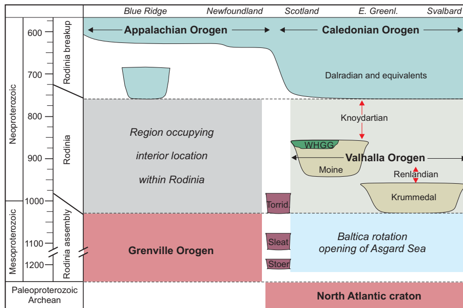
Figure 15. Schematic time-space plot of orogenic successions and events extending from the southeast United States, through the Atlantic provinces of Canada, across Ireland and the UK to East Greenland and Svalbard. The Grenville orogen formed during Rodinia assembly, the Valhalla orogen developed along the margin of an assembled Rodinia, and the Appalachian-Caledonian orogen was initiated during Rodinia breakup. WHGG—West Highland granite gneiss; Torrid—Torridonian.
