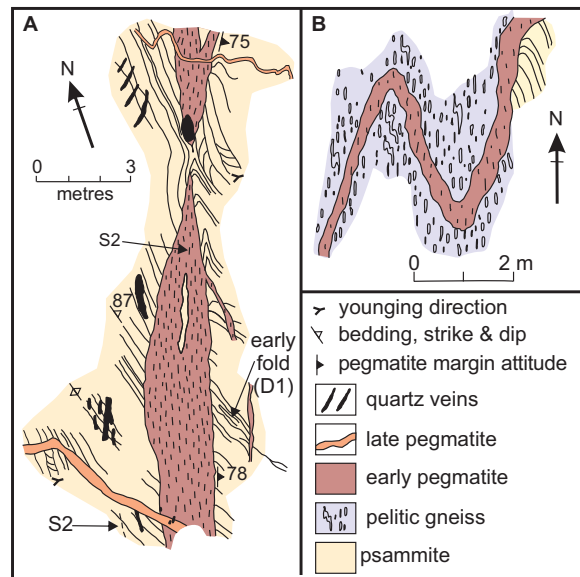
Figure 4. Field sketches of pegmatites intruding Moine sedimentary rocks in the vicinity of Loch Cluanie (after Millar, 1990). (A) Cruachan Coille a'Chait pegmatite (NH 1532 11103) exposed on small hill above the shores of the loch. The pegmatite crosscuts an early D1 fold in psammities of the Loch Eil Group and carries a variable but generally well-developed S2 fabric. (B) Pegmatite exposed on shores of loch (NH 10151 11456) intrusive into pelitic gneisses of the Glenfinnan Group.
