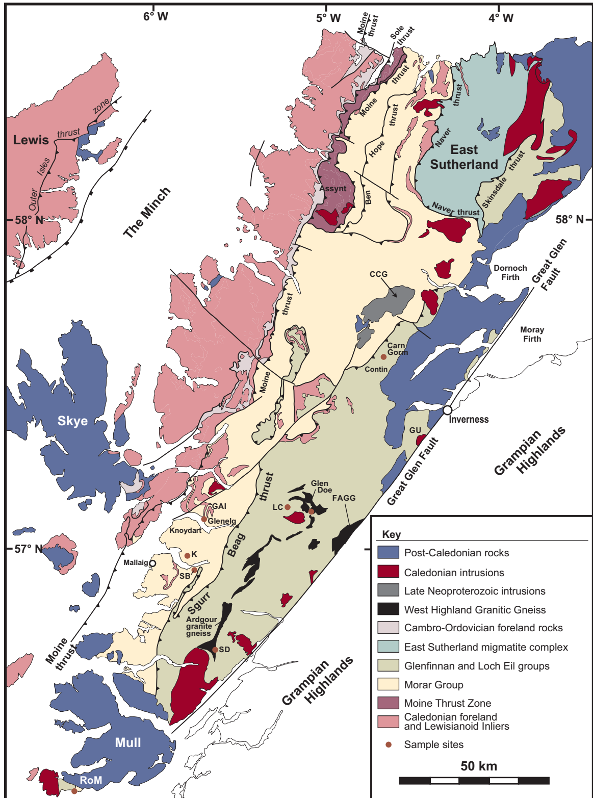
Figure 2. Geological map of northern Scotland (modified from Thigpen et al., 2010) showing the distribution of the Moine Supergroup, consisting of the Morar, Glenfinnan, and Loch Eil groups and East Sutherland migmatites, and the approximate location of analyzed samples (solid pink dot). The Moine Supergroup lies within the Northern Highlands terrane (Fig. 1B), which is separated from the Hebridean foreland to the northwest by the Moine thrust and the Grampian Highlands terrane to the southeast by the Great Glen fault. Abbreviations: CCG—Carn Chuinneag–Inchbae Granite; FAGG—Fort Augustus granite gneiss; GAI—Glenelg–Attadale Inlier; GU—Glen Urquhart; K—Knoydart; LC—Loch Cluanie (including Cruachan Coille a’Chait); RoM—Ross of Mull; SB—Sgurr Breac; SD—Sgurr Dhomhnuill.
