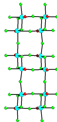
Fig.14 Topology of the [\text{VOF}_3]_n^- “alternating ladder” chain
