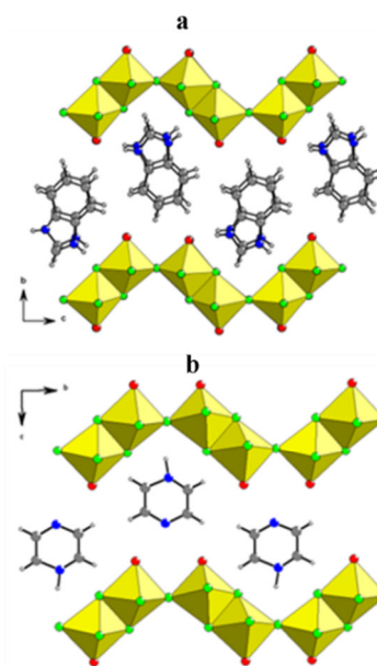
Fig.4 A view of the layer packing in (a) VOF-1 and (b) VOF-2
