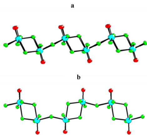
Fig.6 A view of the polymorphic [V 2 O 2 F 5 ] n- layers: (a) found in VOF-3 (b) found in VOF-1 and VOF-2
