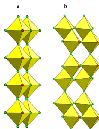
Fig.15 A view showing the standard ladder (a) and the alternating ladder (b)
