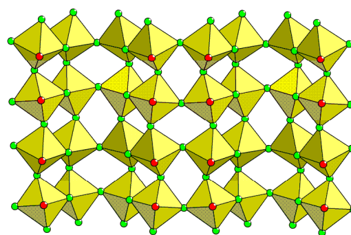
Fig.3 [\text{V}_2\text{O}_2\text{F}_5]_n^+ layer found in VOF-1 and VOF-2
