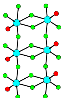
Fig.2 Ladder type [\text{VOF}_3]_n^+ chain
