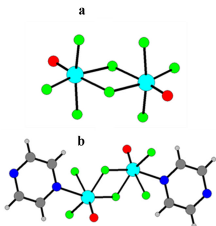
Fig.1 The dimeric [\text{V}_2\text{O}_2\text{F}_8]^{4+} building units observed in (a) all the VOF-n structures except VOF-4 and (b) dimeric unit observed in VOF-4
