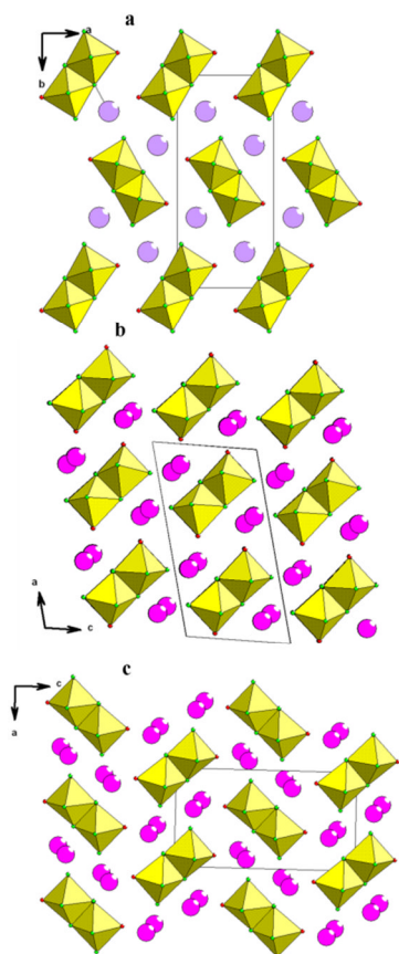
Fig.13 Structures of VOF-10 (a) viewed along the c axis, VOF-11 (b) and VOF-12 (c) viewed along the b axis
