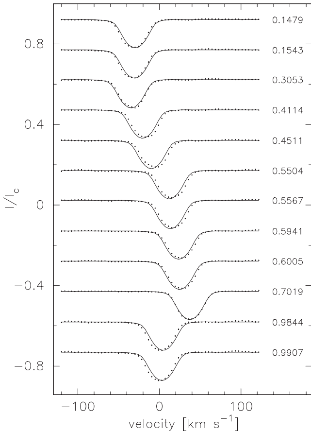
Figure 10. LSD profiles (dots) and unspotted profiles (lines) with the original T_0 .
