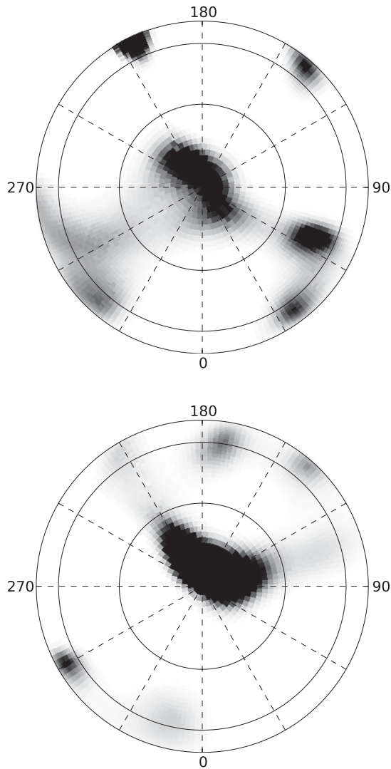
Figure 5. Polar projection of surface images for 2004 February and November.
