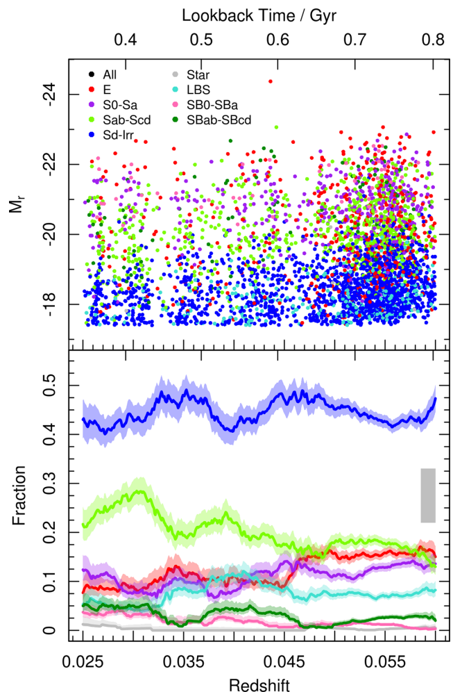
Figure 7. Morphology against redshift. Data points are coloured according to their morphology, as indicated. (top) Absolute r -band Sérsic magnitude as a function of redshift. (bottom) The representative fractions of the total number of galaxies for each morphology, as a function of redshift. Shaded regions indicate \pm 1\sigma binomial confidence intervals (Cameron 2011). These fractions have been constructed using a rectangular kernel with a bandwidth standard deviation of 0.005, as indicated by the width of the grey rectangle inset into the lower plot.
