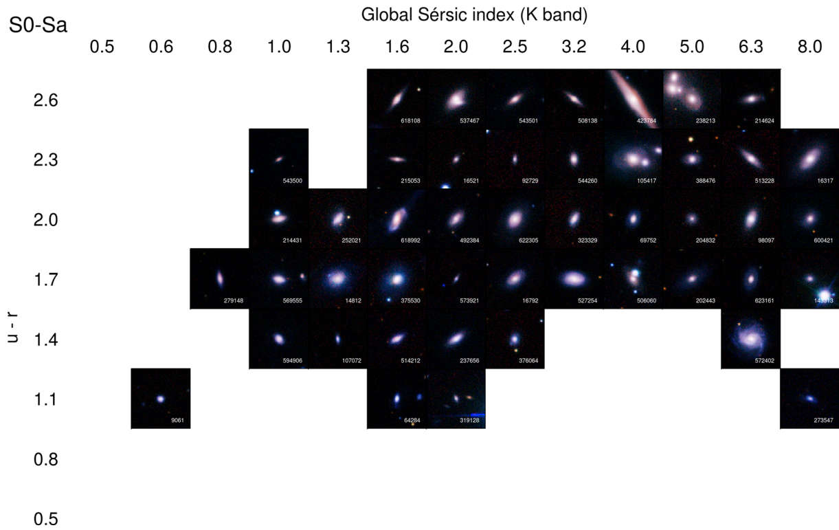
Figure C3. As Fig. C1, but for S0-Sa-type galaxies.
