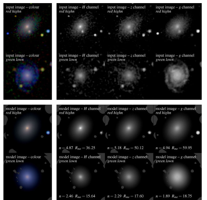
Figure 19. Left: example H_zg images of a red, high- n and a green, low- n galaxy, each with typical dependences of n and R_e on wavelength (they lie at the peaks of their respective distributions in Fig. 18). The images are displayed using the colour-preserving method of Lupton et al. (2004), with an asinh stretch to reveal the full range of surface brightness. The upper panels show the data, while the lower panels show the GALFITM model. Grey regions in the model images indicate where pixels were masked during the fit. Right: individual red, green and blue bands from the colour images, which make it easier to appreciate the relative distributions of the H -, z - and g -band light. For both galaxies, the central region is significantly redder than the outskirts. This is more subtle for the high- n galaxy, as n is stable with wavelength, but still amounts to an increase in R_e by almost a factor of 2 between the H and g bands.
