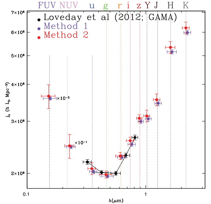
Figure 9. The luminosity density in solar units as measured through the 11 bands via the two methods. The FUV and NUV data points have been scaled as indicated. The data agree to within the errors in all cases. Method 2 is the preferred method now carried forward. Note the data have been jittered slightly in wavelength for clarity. Also shown are the values taken from Table 6 (i.e. [Column 3 + 7 \times Column 4]/8) of Loveday et al. (2012) derived for the ^{0.1}(ugriz) filter set.
