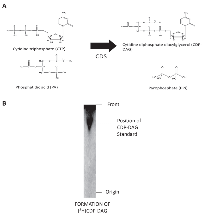
Fig. 1. CDP-DAG synthase activity.
