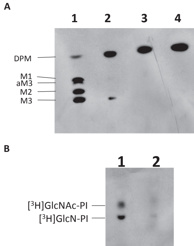
Fig. 6. TbCDS is essential for formation of GPI intermediates.
