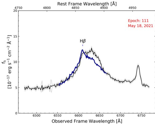
Figure 2. The H\beta spectral region for RM160 in Epoch 111 (2021 May 18, corresponding to MJD 59,352). The dark blue line is the median spectrum computed for the H\beta line centered on the line center and has a total width of 1.5 \times \text{FWHM} reported by Shen et al. (2019). In this particular epoch the H\beta emission-line profile is redder than the median profile. The online version of this figure is an animation. The animation is 1:00 minutes long and shows the time evolution of RM160 for all 127 epochs of spectra beginning on 2013 April 11 and ending on 2022 June 3.
