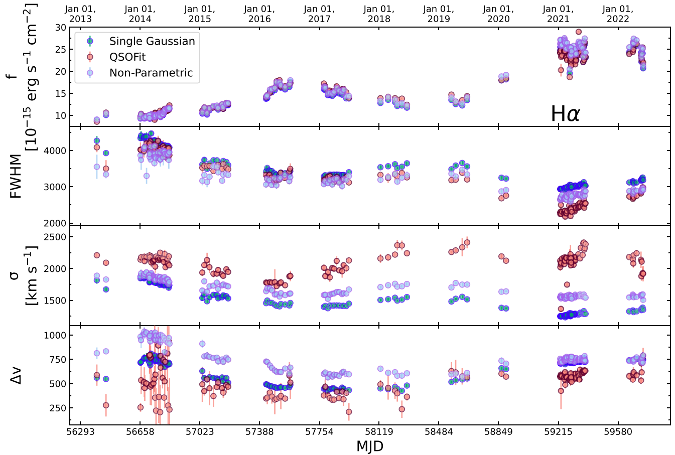
Figure 15. Variability of the H\alpha broad emission-line profile, as quantified by our three fitting methods for the line flux (top row), FWHM (second row), line width \sigma (third row), and the line-center velocity shifts \Delta v (bottom row). The FWHM, line width \sigma , and line-center velocity shift \Delta v are all in units of \text{km s}^{-1} . As for the fit to Mg II, the measured flux and FWHM are consistent across all methods. There are differences in the measured \sigma and \Delta v due to differences in fitting the wings of the line profile, but all three methods find similar qualitative trends of line breathing and shifts in the line center.
