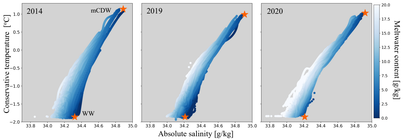
Fig. 4. May-August seal-tag CTD data plotted in temperature-salinity space for each year, colored by meltwater content. Endmember water properties for mCDW and WW used in the meltwater calculations are shown with orange stars.
