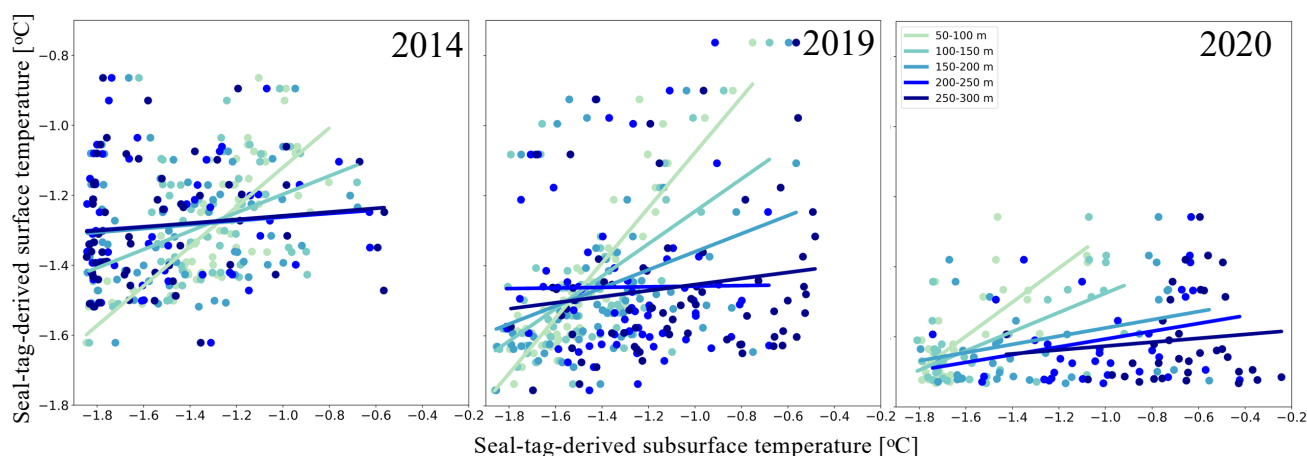
Fig. 7. 2014, 2019, and 2020 seal-derived surface-subsurface water-column correlations for warm profiles. Subsurface temperatures were averaged over 50 m depth intervals (50 – 100 m, 100 – 150 m, 150 – 200 m, 200 – 250 m, 250 – 300 m) and correlated to mean surface (0 – 50 m) temperatures. The equivalent figure for background profiles can be found in the Supplementary Material (Fig. S4).
