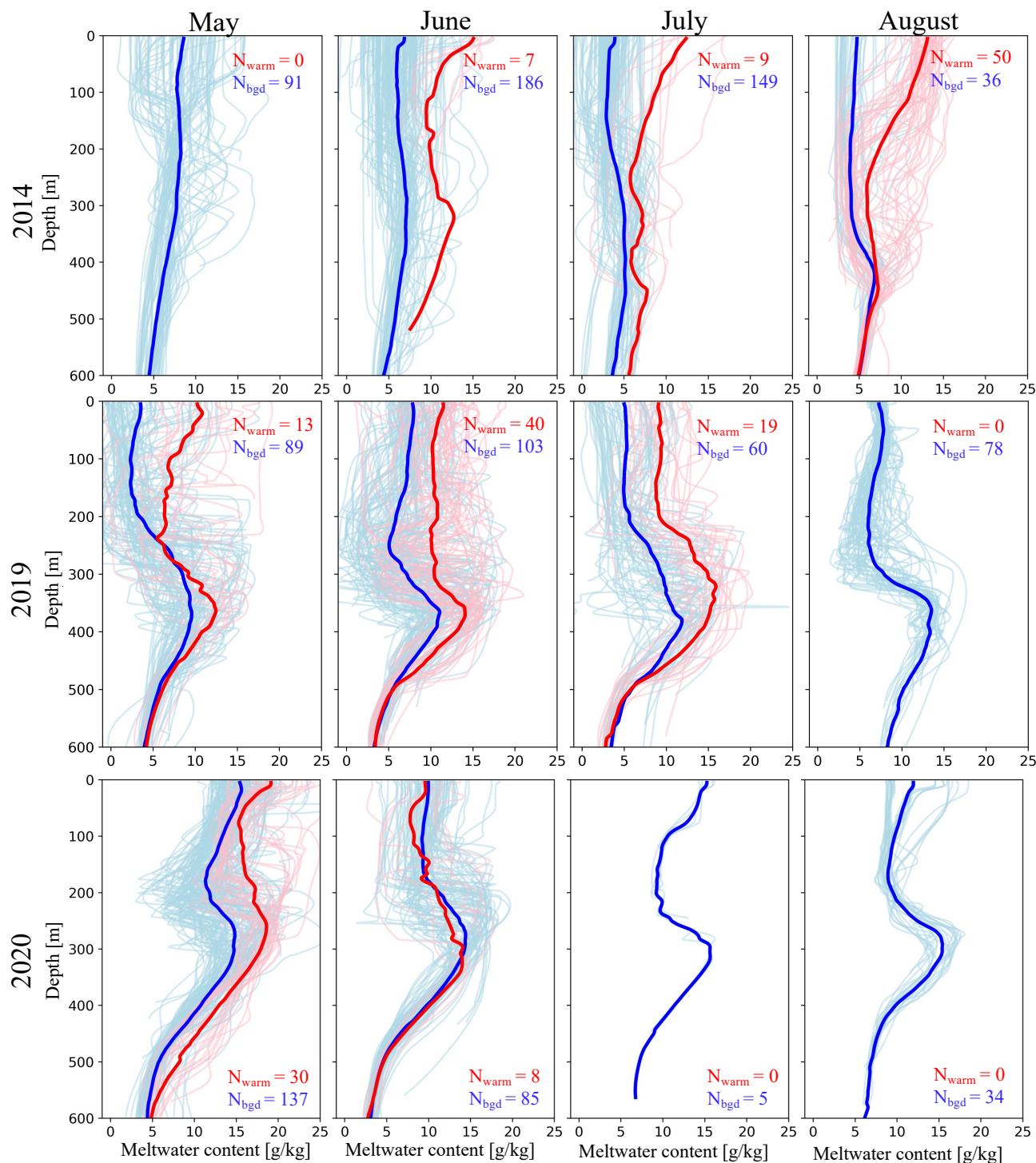
Fig. 6. Seal-tag-derived meltwater profiles near PIGIS front. In all months where there are multiple warm profiles ( N_{warm} = 7 - 50 ) near the ice front, warm profiles corresponded to greater meltwater content than background (bgd) dives. Seal-tag-derived potential density profiles can be found in the Supplementary Material (Fig. S3).
