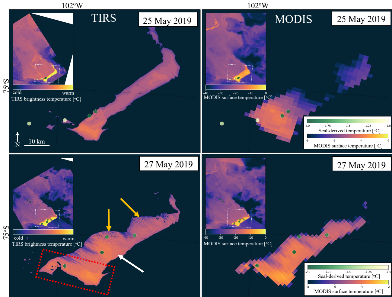
Fig. 3. Comparison of polynya spatial and thermal structure on two days in May 2019 from Landsat 8 TIRS (left column) and MODIS (right column). TIRS (100 m resolution) captures finer-scale detail in comparison to MODIS (1 km resolution). Corresponding seal-derived surface temperatures are overlaid for each day. Mismatch between MODIS- and seal-tag-derived absolute surface temperature retrievals is discussed further in sections III-D and IV-C. Each panel shows the area within the white dashed box on each inset on a narrower temperature scale to highlight the thermal structure within the latent- and sensible-heat polynyas. The red dotted box highlights relatively warm ocean surface temperatures that often extend west of the western margin parallel to the coast and are consistent with surface current flow estimates (e.g., [47]). The white arrow indicates warmer surface temperatures near the middle of the ice front, where strong basal channel outflow has been previously identified [16], [18], [32]. The orange arrows indicate linear features and circular textured areas, consistent with types of sea ice present early in the ice-formation process.
