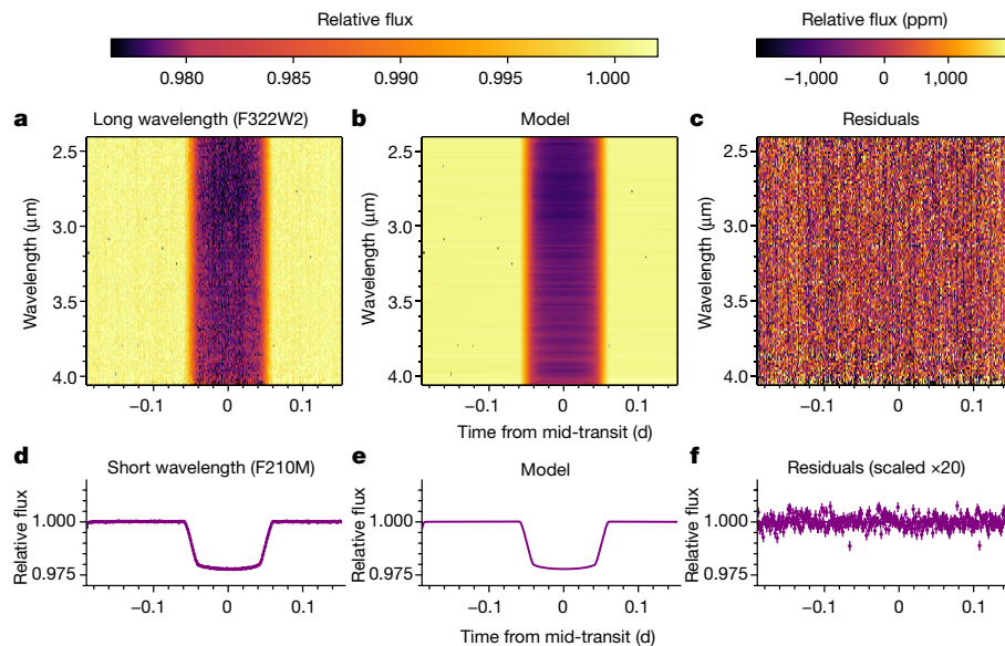
Fig. 1 | The relative brightness of the WASP-39 planetary system as a function of time and wavelength, as measured by NIRCam. a–f , Spectroscopic data (a–c) and the photometric (SW) channel (d–f) for the extracted flux normalized by the median stellar spectrum (a, d), the best-fit transit and
