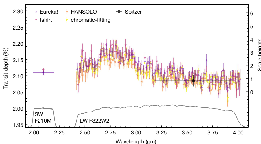
Fig. 2 | The transit spectrum of WASP-39b as measured from JWST’s NIRCam instrument. The coloured points with 1\sigma uncertainties depict our independent analyses of the spectroscopic LW channel (2.420–4.025 μm) and photometric SW channel (2.0–2.2 μm) with their respective throughputs
