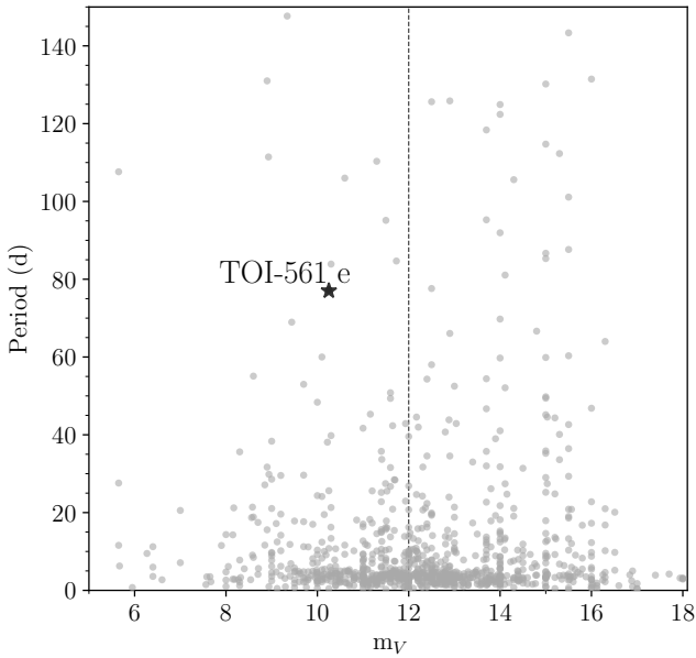
Figure 15. V magnitude versus planetary periods for confirmed transiting exoplanets as reported in the Exoplanets Encyclopaedia catalogue ( http://exoplanet.eu/catalog/ ) in date 18 October 2021. The dashed vertical line marks V = 12 mag. TOI-561 e is one of the few long-period planets orbiting a star bright enough for precise RV characterization.
