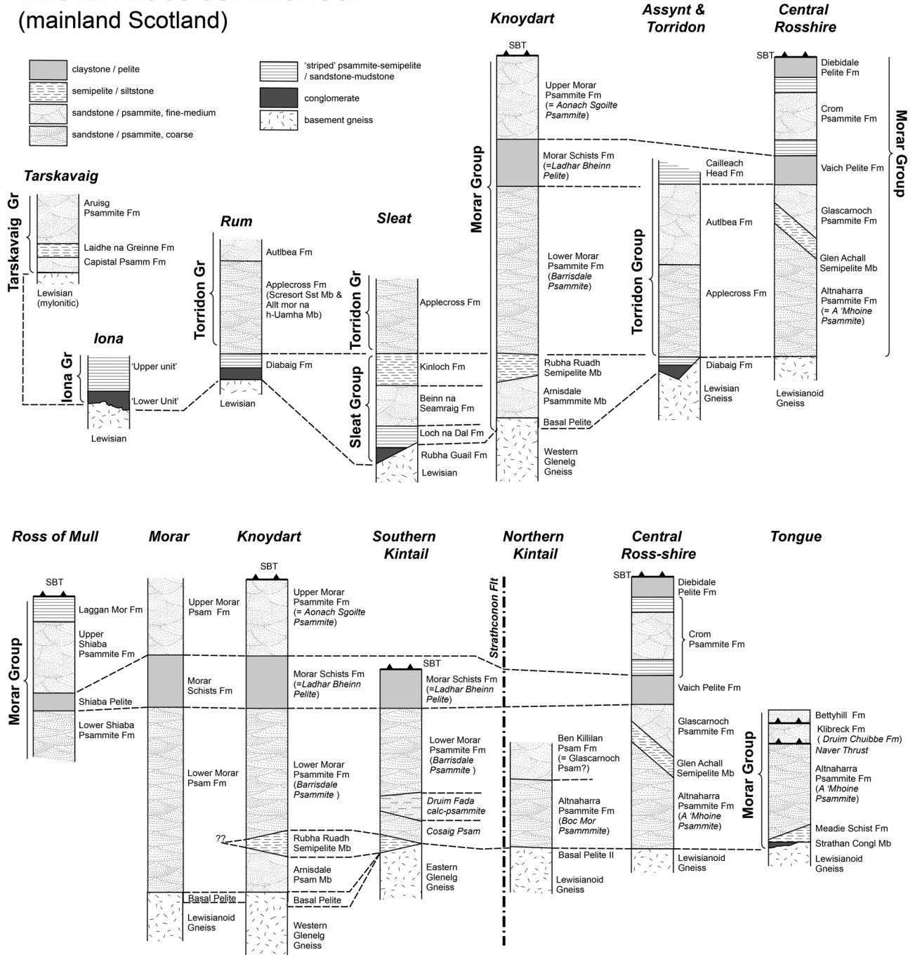
Fig. 5. Stratigraphic correlation chart of the Torridon–Morar groups – Wester Ross Supergroup. References to columns: Tarskavaig: Cheeny and Matthews (1965); Iona: Stewart (2002); McAteer et al. (2014); Rum: Stewart (2002); Sleat: Stewart (1969, 2002). Assynt & Torridon: Stewart (1969, 2002); Ross of Mull: Holdsworth et al. (1987) and this paper. Morar: Johnstone et al. (1969); Powell (1974); Knoydart: Ramsay and Spring (1962); Krabbendam et al. (2014); Southern Kintail: Tanner (1965); Krabbendam et al. (2014, 2018); Northern Kintail: May et al. (1993). Central Ross-shire: Bonsor et al. (2010, 2012); Tongue: Strachan and Holdsworth (1988). Alternative or older names in italics.
