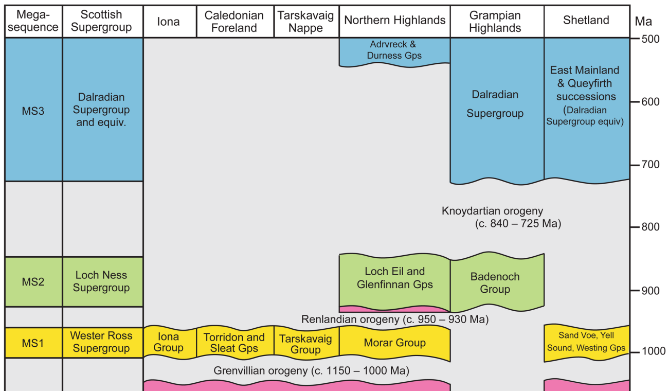
Fig. 11. Revised stratigraphic framework for the Neoproterozoic successions of the Scottish Highlands. The historical terms ‘Torrisonian’ and ‘Moine’ are no longer viable within the emerging understanding of the Neoproterozoic evolution of the North Atlantic region. Two new stratigraphic divisions are erected to retain geological compatibility across the Highlands and North Atlantic: Wester Ross and Loch Ness supergroups.
