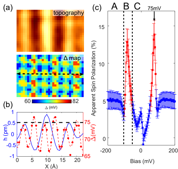
FIG. 4. (a) Topography z(\mathbf{r}) ( V = 200\text{mV} , I = 1\text{nA} ) and spatial map of binding energy \Delta(\mathbf{r}) of the He atom extracted from a spectroscopic map g(\mathbf{r}, V) ( V = 20\text{mV} , I = 1\text{nA} , V_{\text{mod}} = 3.5\text{mV} ) acquired with a setpoint at which the magnetic contrast is not visible in the topography. The \Delta(\mathbf{r}) map shows clear variations between different atomic sites. (b) average profile from z(\mathbf{r}) (blue curve) and along the dashed line from \Delta(\mathbf{r}) (red curve) in a. Besides the difference in \Delta between the hollow and on top sites, a \sim 3\text{mV} modulation is observed between hollow sites with different relative magnetization of tip and sample. (c) The apparent SP of the tunnel junction extracted from the g(\mathbf{r}, V) map. Blue points show true spin polarization, red points show enhancement due to the exchange interaction, leading to a giant apparent SP. There are three regimes: A - He is ejected from the junction, B - He is trapped only at some sites and for one relative magnetic configuration of tip and sample, and C - He remains always in the junction.
