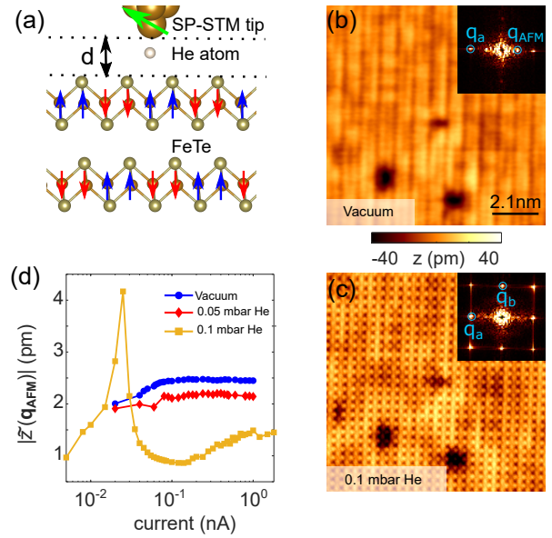
FIG. 1. (a) Schematic of the geometry of the experiment with a He atom as PP in the tunneling junction. d denotes the tip-sample distance (see suppl. section S2A). Magnetic moments in \text{Fe}_{1+x}\text{Te} are drawn vertical for clarity, but point into the plane of the figure in reality[9]. (b) Topographic SP-STM image z(\mathbf{r}) of \text{Fe}_{1+x}\text{Te} measured in vacuum ( V = 50\text{mV} , I = 100\text{pA} ). The bi-collinear AFM order of \text{Fe}_{1+x}\text{Te} is seen as a stripe-like modulation. Inset: Fourier transformation |\tilde{z}(\mathbf{q})| . (c) z(\mathbf{r}) image recorded with the same tip and in the same location as (b) after admission of He into the vacuum chamber at a partial pressure p_{\text{He}} = 0.1\text{mbar} . The magnetic contrast is hardly visible. Inset: corresponding |\tilde{z}(\mathbf{q})| . (d) Amplitude |\tilde{z}(\mathbf{q}_{\text{AFM}})| of the Fourier peak associated with the AFM order at different tunneling currents for a bias voltage of V = 50\text{mV} in vacuum, and with p_{\text{He}} = 0.05\text{mbar} and 0.1\text{mbar} .
