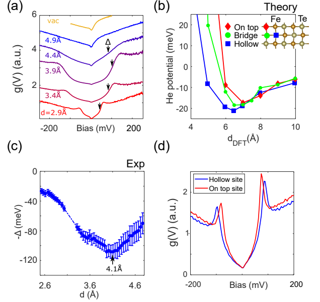
FIG. 2. Spectroscopy in He at p_{\text{He}} = 0.1\text{mbar} . (a) Differential conductance spectra g(V) ( V = 50\text{mV} , I_s = 80\text{pA} , V_{\text{mod}} = 5\text{mV} ) recorded at different d in the presence of He. A g(V) spectrum taken in vacuum (yellow) is also shown ( V = 100\text{mV} , I_s = 300\text{pA} , V_{\text{mod}} = 1\text{mV} ). Spectra are vertically offset for clarity and normalized at V = 250\text{mV} . (b) DFT calculation of the trapping potential for the He atom in the junction for different adsorption sites. (c) The gap size \Delta(d) , plotted as -\Delta(d) , extracted from g(V) spectra (defined as the inflection point at the gap edge) as a function of d . \Delta(d) exhibits a similar functional form as the potential of the He atom found in the DFT calculation in (b). (d) g(V) spectra recorded with the tip positioned above the hollow (blue) and on top site (red) showing a larger gap for the hollow site ( V = 20\text{mV} , I = 1\text{nA} , V_{\text{mod}} = 3.5\text{mV} ).
