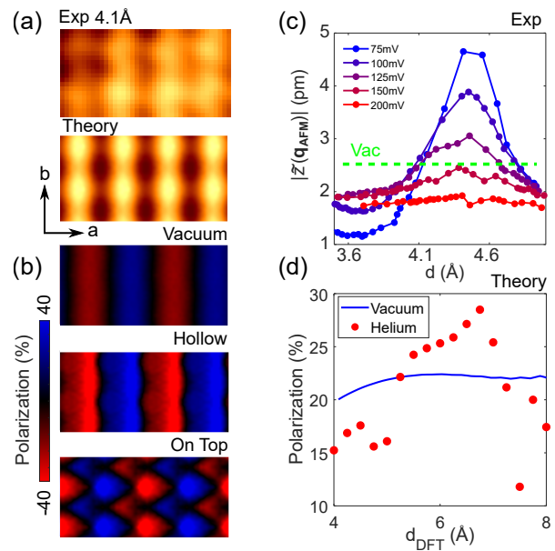
FIG. 3. (a) z(\mathbf{r}) image for d = 4.1\text{\AA} ( V = 50\text{mV} , I = 30\text{pA} ) and the simulated topography for d_{\text{DFT}} = 7.6\text{\AA} for comparison. (b) calculated SP at the same d_{\text{DFT}} for vacuum tunneling and for a layer of He in the hollow and the on top sites. The largest magnetic contrast is observed for He in the hollow site. (c) Amplitude |\tilde{z}(\mathbf{q}_{\text{AFM}})| of the magnetic order as a function of d and for a range of voltages V . The green dashed line represents the value for vacuum tunneling. (d) The SP P extracted from the amplitude of the magnetic order in the simulated images. Red points are extracted from our model accounting for the He atom probing different sites during the measurement (for details see suppl. S1B). The blue curve is the intensity of the magnetic order for a vacuum junction.
